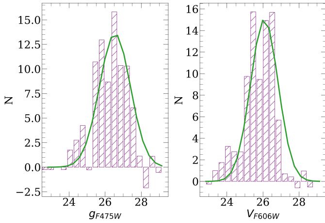
Fig. 11. Final GCLF which has been corrected for completeness, and fitted with a Gaussian (green line).
