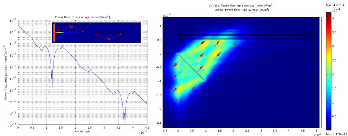
Figure 2.1 \text{Si}_3\text{N}_4 200nm gratings channel with evaporated Gold at each end (50nm residual diameter), He II line, TM.
