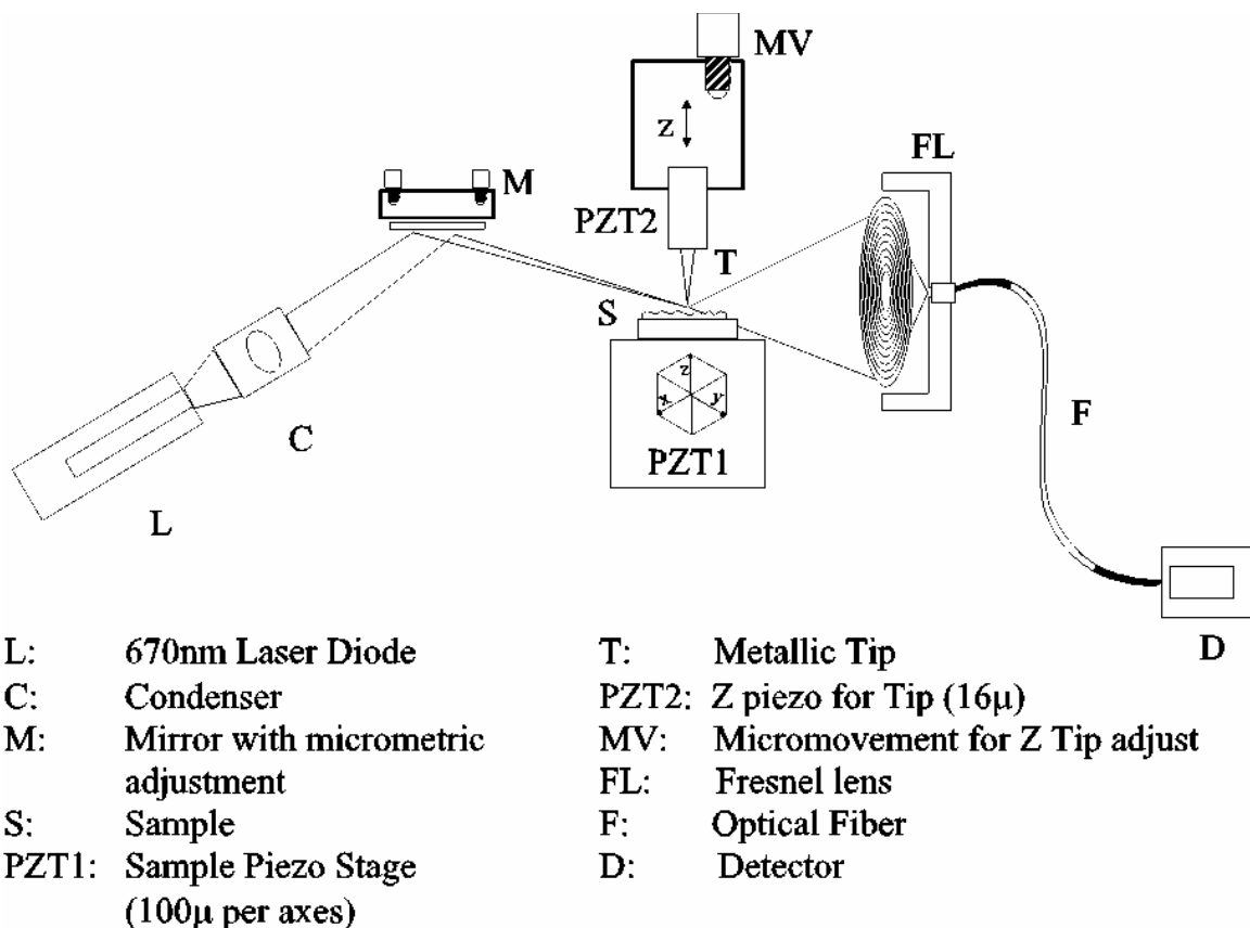
Figure 2.1. View of the optical test bench
