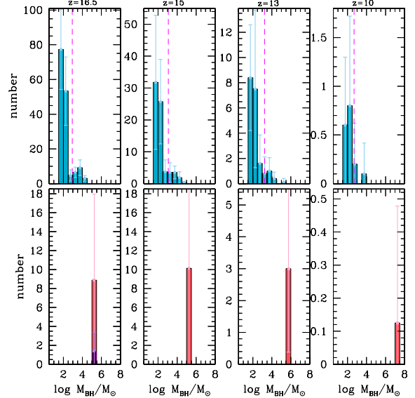
Figure 3. Mass distribution of accreting light (upper panels) and heavy (lower panels) BH seeds at 4 different redshifts: z=16.5, 15, 13 and 10 . The dashed lines in the upper panels indicate the average mass of ILS at the corresponding z .
