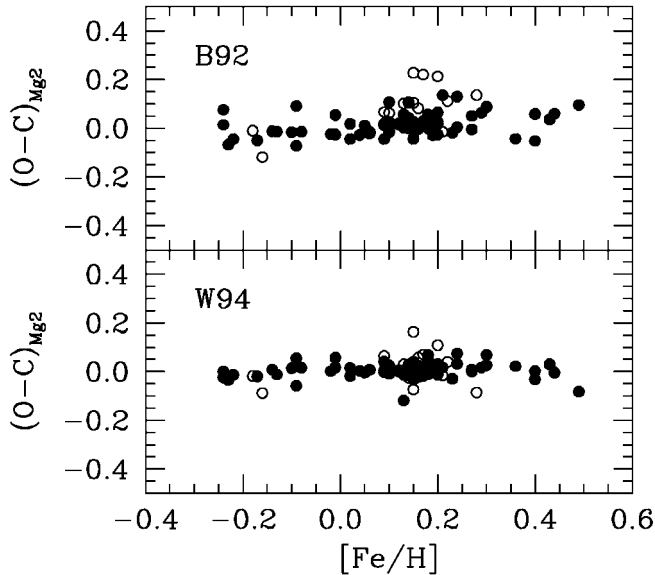
FIG. 6.— Mg_2 index residuals (in the sense [observed – computed]) with respect to B92 and W94 fitting functions vs. metallicity for the fair (filled circles) and the extended (open circles) samples. Both (O - C) distributions are consistent with a zero average. Point spread for the fair sample across the B92 fitting function is \sigma(Mg_2) = \pm 0.049 mag, and \sigma(Mg_2) = \pm 0.031 mag with respect to W94.
