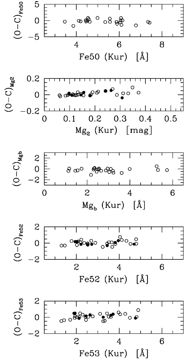
FIG. 2.—Index calibration to the standard Lick system, after eq. (4), for the fiducial model atmospheres of the 25 primary calibrators in common with W94 (open circles) and the nine stars from B92 and B94 (filled circles). The (O - C) residuals are in the sense [synthetic – standard]. Point scatter is \sigma(\text{Fe50}) = \pm 0.70 Å, \sigma(\text{Mg}_2) = \pm 0.029 mag, \sigma(\text{Mg b}) = \pm 0.40 Å, \sigma(\text{Fe52}) = \pm 0.27 Å, and \sigma(\text{Fe53}) = \pm 0.34 Å. These higher values, compared with those of the observations (see Fig. 1), give a measure of the residual variance of the theoretical models due to the intrinsic limitation of the input physics.
