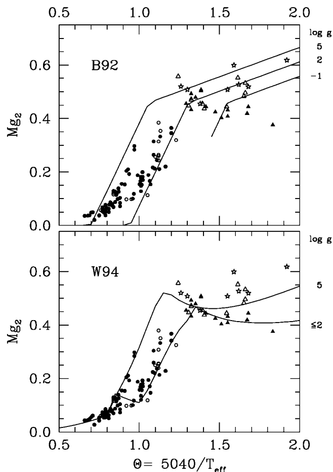
FIG. 10.— Mg_2 data distribution for the fair (filled circles) and extended (open circles) samples vs. B92 and W94 fitting-function predictions (solid lines). To ease comparison, observations have been corrected to [Fe/H] = 0 by subtracting the corresponding [Fe/H] polynomial term of each fitting set. In order to span the whole range of temperature, Mg_2 measurements of eight Gliese red dwarfs from B92 (stars) have also been added in both panels together with 10 M dwarfs from the Gorgas et al. (1993) sample (open triangles). The low-gravity range is also spanned by a set of 16 field M giants with T_{\text{eff}} < 3900\text{ K} , from W94 (filled triangles). The B92 and W94 fitting functions have been computed for \log g = 5.0, 2.0 , and -1.0 dex, as labeled in each panel. Below 3900\text{ K} the W94 fit is insensitive to stellar gravity, so the \log g = 2 and -1 curves merge. A solar metallicity is assumed throughout in the models.
