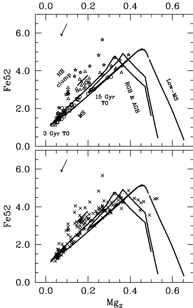
FIG. 11.— Mg_2 vs. Fe52 distribution for (upper panel) the 87 stars with fiducial atmosphere parameters in the extended sample and for (lower panel) the global observed sample of 139 stars. Stars in the upper panel are marked according to their surface gravity (stars: \log g < 2.0 ; open triangles: 2.00 \leq \log g \leq 3.5 ; open circles: \log g > 3.5 ). The theoretical locus for 3 and 15 Gyr old simple stellar populations with [Fe/H] = +0.2 from Buzzoni (1989) is superposed on the data, and main evolutionary phases are labeled (main sequence [MS], turnoff point [TO], red giant branch [RGB], asymptotic giant branch [AGB], and horizontal branch [HB]). The vector top left in each panel is the expected variation in the observed indices for a change in [Fe/H] of -0.5 dex.
