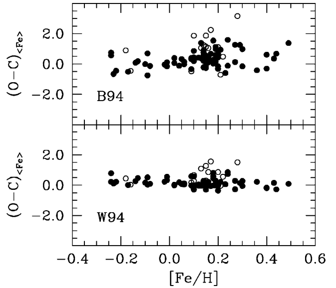
FIG. 7.—Same as Fig. 6 but for the combined Fe index \langle Fe \rangle = (Fe52 + Fe53)/2 . Point spread of the fair sample (filled circles) with respect to the zero-average (O - C) is \sigma(\langle Fe \rangle) = \pm 0.61 Å compared with B94 and \sigma(\langle Fe \rangle) = \pm 0.30 Å with respect to W94.
