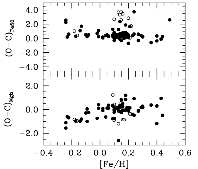
FIG. 8.—Same as Fig. 6 but for the Fe50 and Mg b indices. The (O - C) residuals are computed with respect to the W94 fitting functions. Point spread for the fair sample (filled circles) with respect to the zero-average (O - C) is \sigma(Fe50) = \pm 0.95 Å, and \sigma(Mg\ b) = \pm 0.83 Å. A trend with [Fe/H] (opposite for Fe50 and Mg b ) appears in the data.
