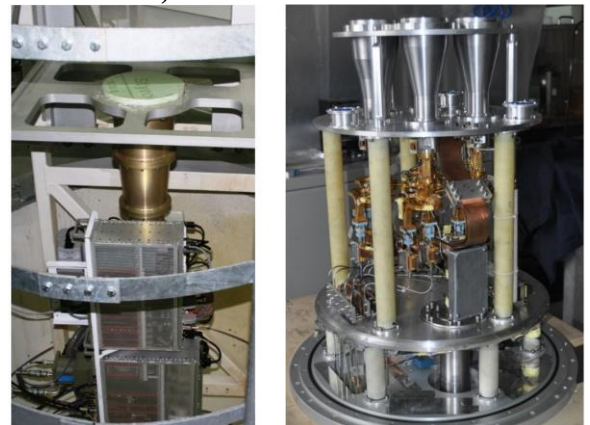
Figure 5. Monofeed High-C-band receiver installed at the BWG focus (left); view of the cryogenic assembly of the K-band multibeam receiver (right).
