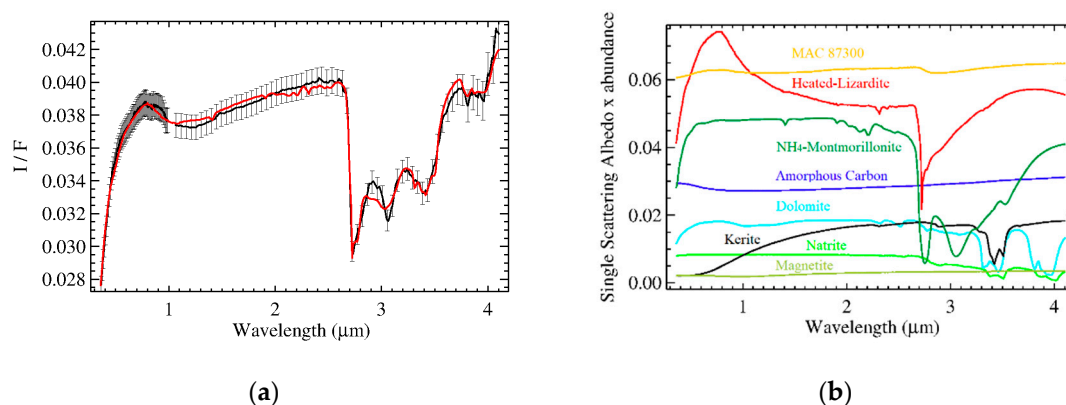
Figure 6. Panels (a): measured (black) and modeled (red) average spectrum of Ceres in terms of I/F ( r \times \pi ) of the organic-rich spectra from area A and area B, respectively. Error bars indicate calibration uncertainties. In panel (b), the relative SSA of each endmember scaled for their respective abundance (relative cross section): MAC 87300 (orange), \text{NH}_4 -montmorillonite (dark green), heated lizardite (red), amorphous carbon (blue), dolomite (cyan), antigorite (purple), natrite (light green), magnetite (pickle green), kerite (black).
