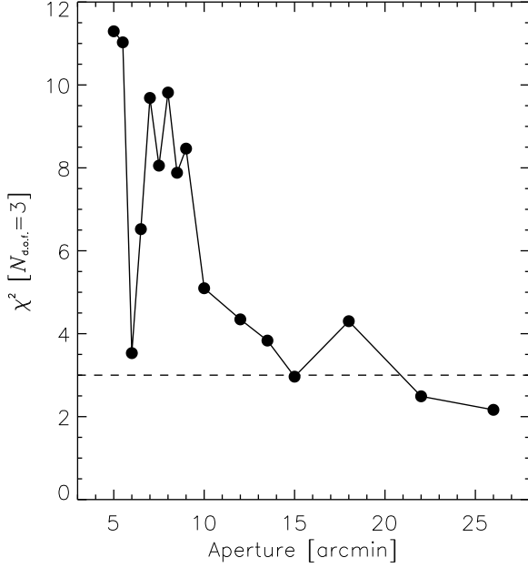
Fig. 9. Evaluations of the \chi^2 statistic of the w_{\text{los}}^{\text{T,rec}}(r) correlation function (with respect to the null hypothesis) for different angular apertures. Only results for the foreground-cleaned SEVEM map are shown. There is evidence for kSZ signal in a wide range of apertures above the FWHM, with a local maximum close to 8 arcmin. This roughly corresponds to a radius of 0.8 h^{-1} \text{ Mpc} from the CG positions at the median redshift of the sample.
