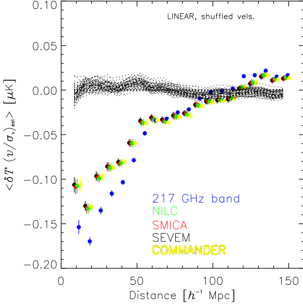
Fig. 7. Same as in Fig. 6, but with the null correlation functions (displayed by dotted lines) being estimated after assigning the recovered linear velocity estimate of a given CG to any other CG in the sample (that is, by v_{\text{los}}^{\text{rec}} “shuffling”). Only the LINEAR approach is displayed in this plot.
