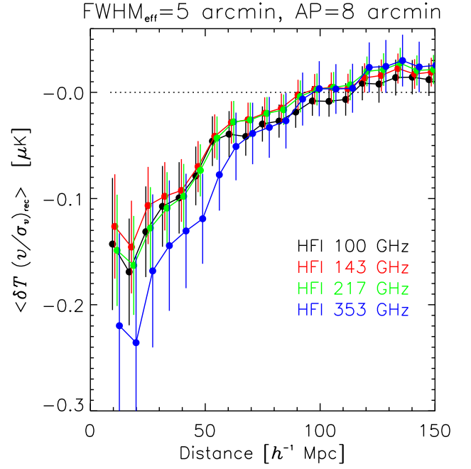
Fig. 10. Variation of the recovered w_{\text{los}}^{\text{T,rec}}(r) correlation function for the four lowest frequency raw HFI maps after an effective convolution by a Gaussian beam of \text{FWHM} = 5 \text{ arcmin} . Error bars here are computed in the same way as in Figs. 6 and 8.
