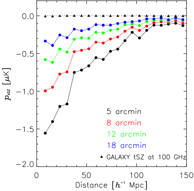
Fig. 5. (Filled circles): Measured kSZ pairwise momentum for the kSZ map derived from the CLUSTER simulation after considering different radial apertures on a subset of clusters in the mass range (1\text{--}2)\times 10^{14} h^{-1} M_{\odot} . (Black triangles): Pairwise momentum computed from the GALAXY mock catalogue (filled triangles) after assigning these galaxies a tSZ amplitude following a mass scaling inspired by the tSZ measurements of the CGC given in Planck Collaboration Int. XI (2013).
