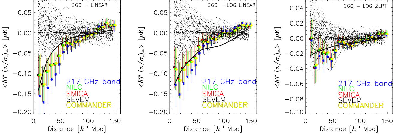
Fig. A.1. Measured cross-correlation function between the kSZ temperature estimates and the recovered radial peculiar velocities, w^{\text{T},v_{\text{los}}^{\text{rec}}}(r) , according to the three adopted approaches, LINEAR (left panel), LOG-LINEAR (middle panel), and LOG-2LPT (right panel). The velocities are normalized with their rms dispersion \sigma_v = 230, 310 , and 200 \text{ km s}^{-1} from left to right, respectively. We use an aperture of 8 arcmin when estimating kSZ temperature fluctuations. Filled coloured circles correspond to w^{\text{T},v_{\text{los}}^{\text{rec}}}(r) estimates from different CMB maps (SEVEM, SMICA, NILC, COMMANDER, and the HFI 217 GHz map). The dotted lines display the null estimates obtained after computing kSZ temperature estimates for rotated positions on the SEVEM map, and the thick dashed line displays the average of the dotted lines. Error bars are computed from these null estimates of the correlation function. The solid line provides the best fit to the data of the theoretical prediction for w^{\text{T},v_{\text{los}}^{\text{rec}}}(r) obtained from the GALAXY mock catalogue. These predictions are obtained using only a relatively small number of mock halos, and hence their uncertainty must be considered when comparing to data.
