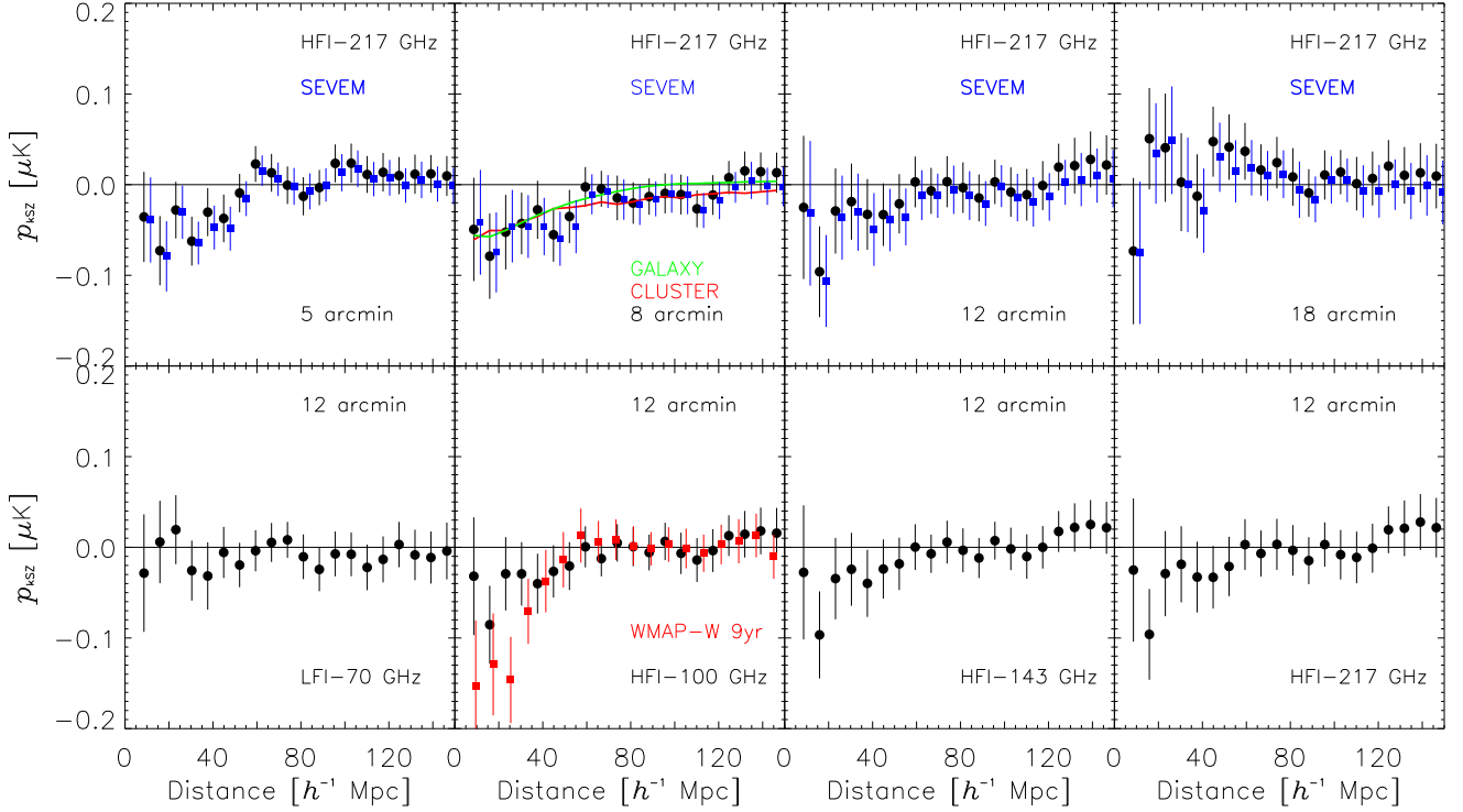
Fig. 4. Computation of the kSZ pairwise momentum for the CGC sample. The top row, from left to right, displays the results for different aperture choices on the raw HFI 217 GHz map, namely 5, 8, 12, and 18 arcmin. The top row also shows the analysis for the foreground-cleaned SEVEM map, displayed with blue squares. The fit to the pairwise momentum templates from the CLUSTER catalogue is also displayed by the solid red line, and the GALAXY catalogue by the green line. The bottom row presents the results at a fixed aperture of 12 arcmin for different frequency maps, including WMAP-9 W-band data (red squares).
