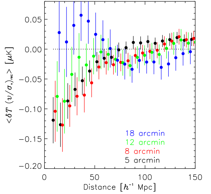
Fig. 8. Dependence on the aperture radius of the w^{\text{T},v_{\text{los}}^{\text{rec}}}(r) correlation function obtained in the LINEAR approach for the SEVEM map. Error bars are estimated from the rms of the null correlation functions computed from rotated kSZ temperature estimates.
