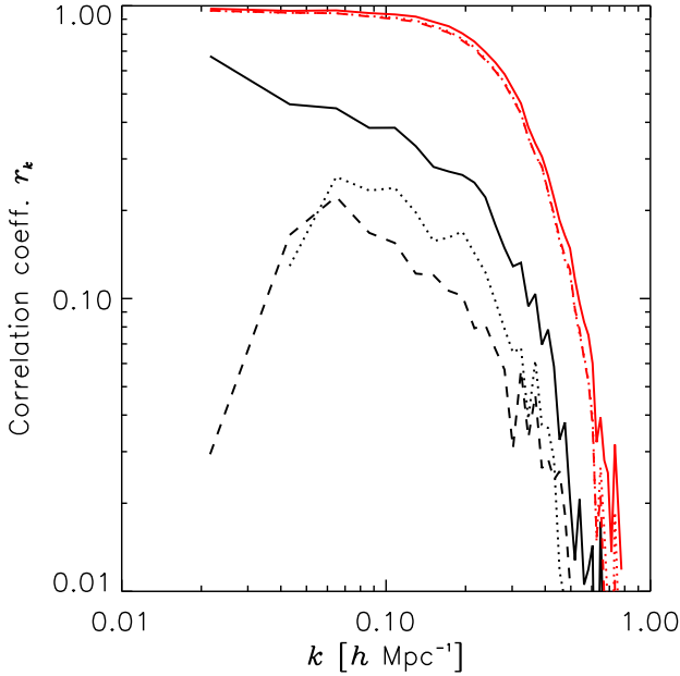
Fig. 3. Correlation coefficient of the recovered line-of-sight velocities with the actual ones in our GALAXY mock catalogue. Solid, dotted, and dashed lines refer to the LINEAR, LOG-LINEAR, and LOG-2LPT approaches, respectively. The red lines consider the ideal scenario without any sky mask or selection function, while the black ones are for the same sky mask and selection function present in the real CGC.
