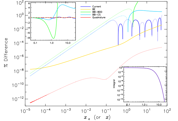
Fig. B.1. Comparison between the results of various approximations and accurate numerical integrations of Eq. (B.1). The bottom-right inset gives the numerical result derived with the NAG routine D01AJF with a relative accuracy of 10^{-12} in the case of the blackbody spectrum. The main plot reports the per cent difference of various estimations of Eq. (B.1) with respect to the NAG D01AJF result for the blackbody spectrum: the approximation presented here (Current, see Eq. (B.5)); the NAG D01AJF result but for a pure BE spectrum with \mu_0 = 1.4 \times 10^{-5} (BE); the approximations reported in Burigana et al. (1991a) (BB-BDD, see Eq. (B.3)) and in Chluba & Sunyaev (2012) (BB-CS, see Eq. (B.4)); the numerical result derived with a Gaussian quadrature scheme (Press 1992) with the accuracy parameter ( EPS ) set to 10^{-9} and 2048 points in the case of the blackbody spectrum. Solid lines (or dots) correspond to positive (or negative) values. The top-left inset displays the same results of the main plot, but in a restricted frequency range and with a linear scale on the y-axis. See also the legend and the text.
