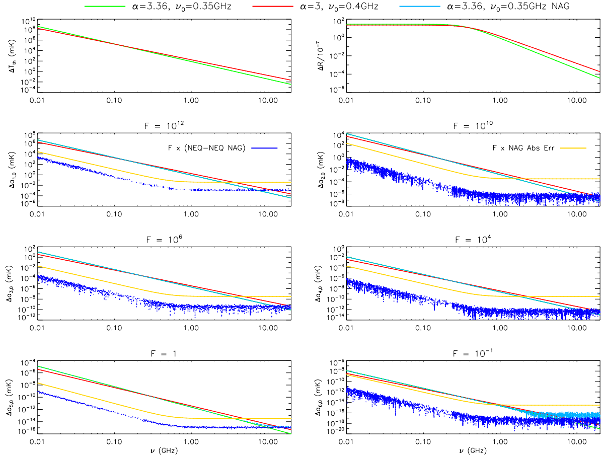
Fig. 1. \Delta T_{\text{th}} , \Delta R and \Delta a_{\ell,0} from \ell = 1 to \ell_{\text{max}} = 6 for the considered non-equilibrium models. Solid lines (or dots) correspond to positive (or negative) values. Green and light blue lines are essentially superimposed up to \ell = 4 , where only one of the two lines can be appreciated. Their difference multiplied by a factor F to have values compatible with the adopted range is displayed by the blue lines. Yellow lines refer to the nominal integration error quoted by the routine DOI AJF , again multiplied by the factor F . See also the legend and the text.
