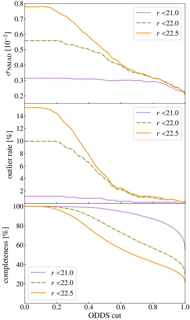
Fig. 11. Dependence of the Normalized median absolute deviation of photo- z errors ( \sigma_{\text{NMAD}} ) (top panel), outlier rate (middle panel), and completeness (bottom panel) on the ODDS parameter for different r -band cuts.
