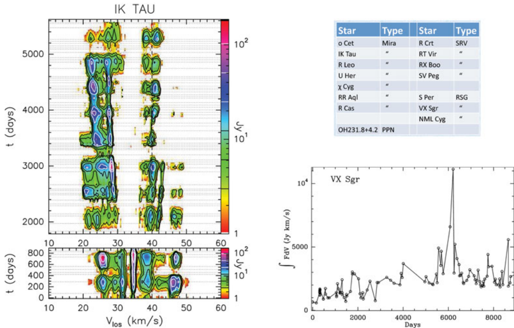
Figure 1. a (left). Flux density versus velocity, as a function of time, for IK Tau. Each horizontal dotted line indicates an observation (spectra within 4 days from each other were averaged). Data are resampled to 0.3 km/s and only emission at levels \geq 3\sigma is shown. Day 0 = 12/12/95. b (top right). Observed targets. c (bottom right). A flare in VX Sgr; the integrated flux increased by a factor of 4–5, and declined, in a period of about 2.4 yrs (2003–05). Note the general increase of integrated emission over time (by a factor of \geq 2 ). Day 0 = 28/3/87.
