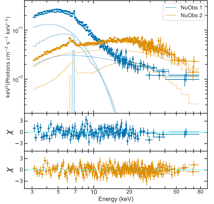
Figure 5. Soft state (blue) and hard state (orange) spectra with best-fit models and model components shown with solid and dashed lines, respectively. FPMA spectra are shown with \times 's while FPMB spectra are shown with filled circles. The soft state spectrum is described well by a Comptonized disk blackbody, while the hard state spectrum does not require a disk component. Instead, the hard state spectrum is described well by a power law with a high energy cutoff. Both models are improved by the addition of relativistic disk reflection as well as a narrow Fe line component. The lower two panels show the residuals resulting from the model fits in units of \chi = (\text{data} - \text{model})/\text{error} .
