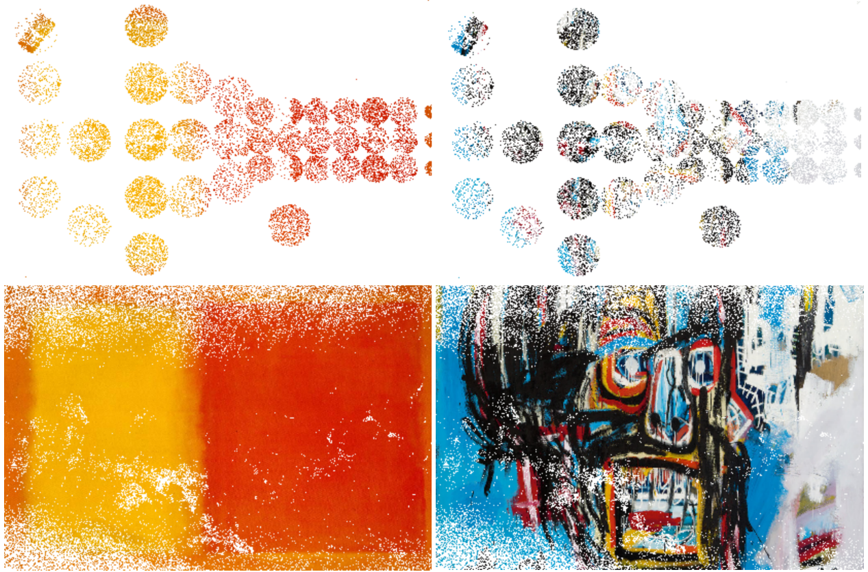
Figure 1: The transition from the top to bottom panels represents the transformative view of the Galaxy that will be provided by the contiguous, continuous mapping of Sloan V’s Milky Way Mapper. At top is the (pencil-beam) sampling of the groundbreaking APOGEE survey, for paintings by Mark Rothko at left and Jean-Michel Basquiat, at right. If the Milky Way is structured on the scales of Basquiat (as Gaia results indicate) then our dense mapping that will be carried out in the 2020’s will revolutionize our picture of the Galaxy. If our Galaxy is sparsely structured, the gains in dense sampling will be more modest. (In practice, vast samples and many more dimensions of information get to a level of detail that even this striking illustration only partly indicates). Image credit: Jonathan Bird
