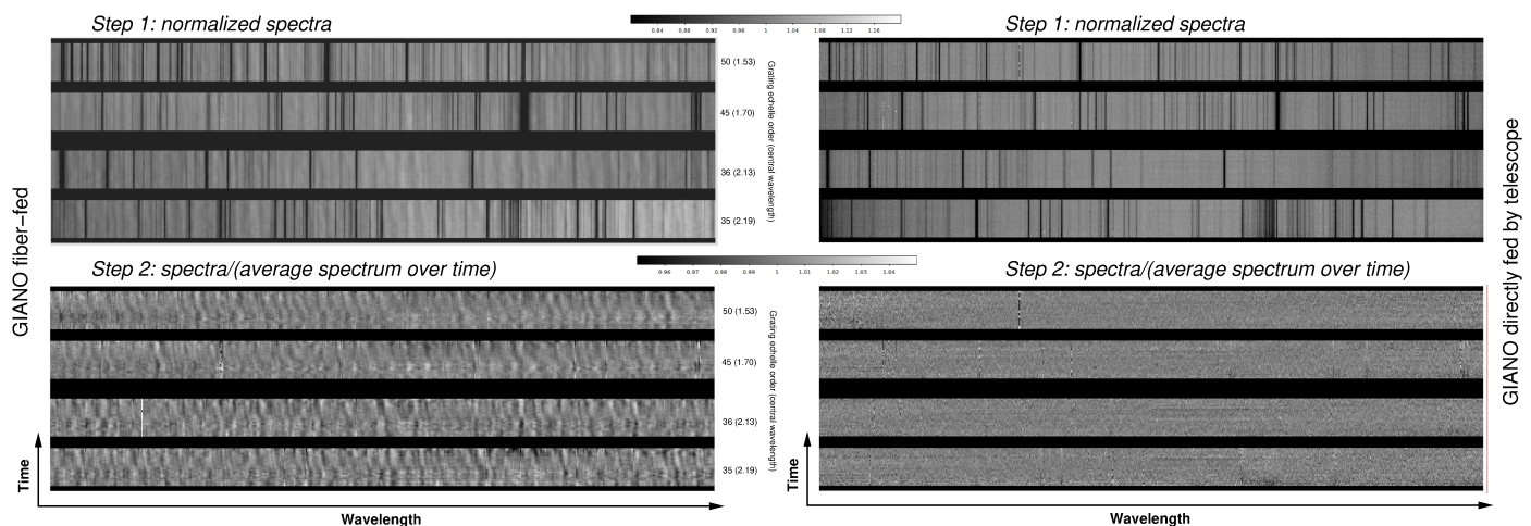
Fig. 1. Times-series spectra of stars collected with the GIANO spectrometer. The left- and right-hand panels show the data collected with and without fiber feeding, respectively. Modal noise causes the wavy pattern clearly visible in the data taken with fibers.
