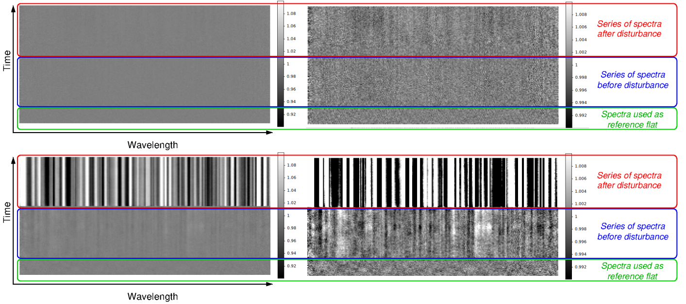
Fig. 3. Example of 2D times-series spectra with different illuminations of the fiber. Top panel: uniform illumination (overfilled). Bottom panel: under-filled illumination. The left- and right-hand panels show the same data with different gray scale limits: \pm 10\% and \pm 1\% , respectively.
