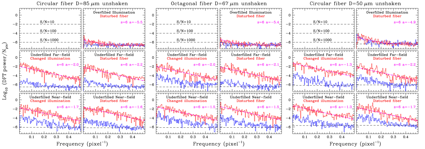
Fig. 4. Digital Fourier transform spectral analysis of data taken with different fibers without mechanical agitator. See text (Sect. 4) for details
