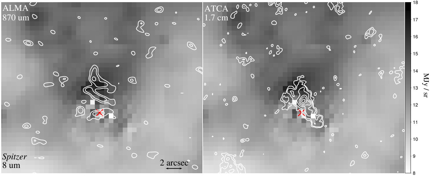
Fig. 7. Residuals from the 8 \mu\text{m} IRAC image after point-source subtraction. The white contours are the [2, 3, 4 \sigma ] ALMA Band 7 emission ( left ) and the [2, 3, 4, 5, 6, 7 \sigma ] ATCA 17 GHz emission ( right ). North is up and east is left. The red cross indicates the position of the star.
