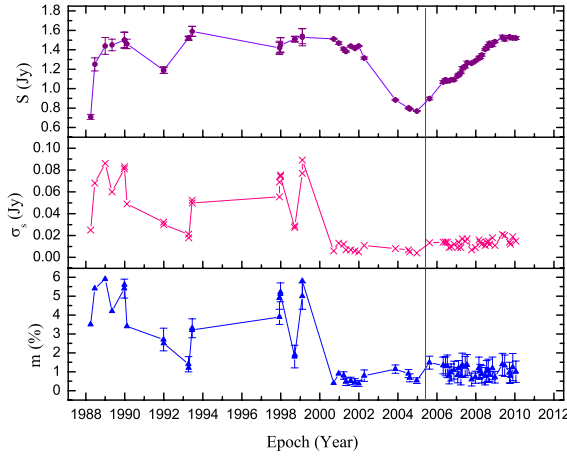
Fig. 2. Upper panel: total flux density of S4 0917+624 at \sim 5 GHz in the IDV observations; middle panel: the rms flux density at \sim 5 GHz; lower panel: IDV modulation index at \sim 5 GHz versus time, the error on m is the mean modulation index of calibrators. Urumqi data from August 2005 to January 2010 are shown to the right of the vertical line.
