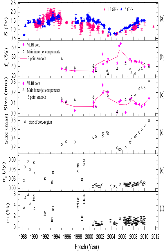
Fig. 5. From top to bottom: a) total flux density at 14.5 GHz (from the UMRAO database) and at 4.8 GHz (from the UMRAO and the IDV observations); b) flux ratio ( f_c ) of the VLBA core or inner-jet component to total flux density of S4 0917+624; c) angular size of the VLBA core or inner-jet components at 15 GHz; d) size of the broad “core region” fitted with a single Gaussian model; e) rms flux density at 5 GHz versus time; f) IDV modulation index at 5 GHz versus time.
