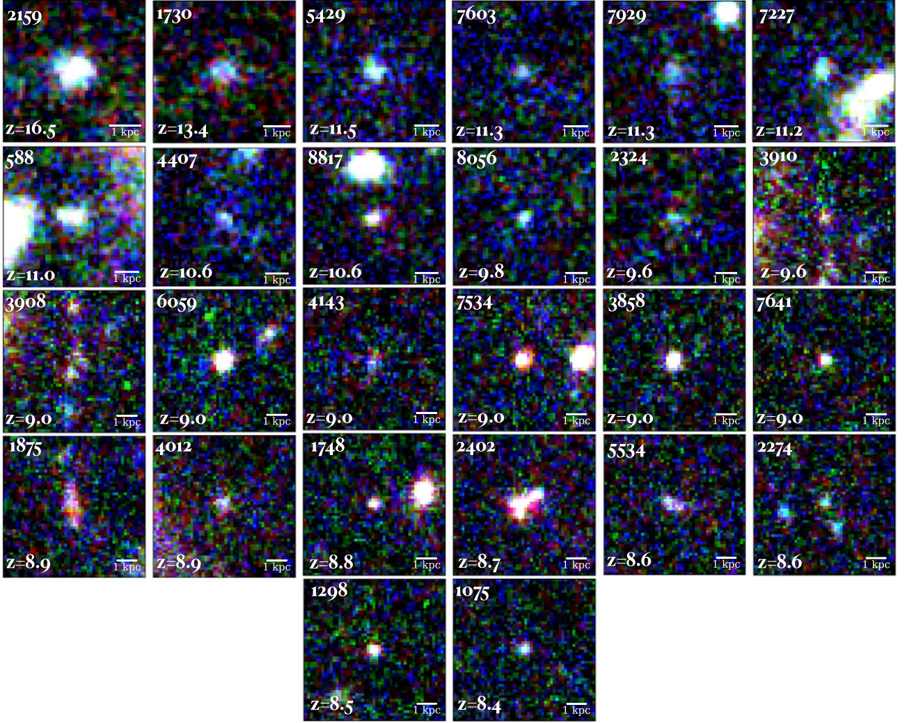
Figure 4. Montage of images for the galaxy candidates identified here. For each galaxy, the image shows as blue–green–red the three NIRCcam bandpasses closest to the Ly \alpha break, which includes F150W, F200W, and F277W for galaxies at z = 9 ; F200W, F277W, and F356W for galaxies in the z = 10 –12 samples; and F277W, F356W, and F444W for galaxies in the z \geq 12 samples. In each case, the images are 1''.5 \times 1''.5 . The inset scale bar shows 1 (physical) kpc. We list the numerical IDs and best-fitting photometric redshift values (the redshift uncertainties are listed in Table 2).
