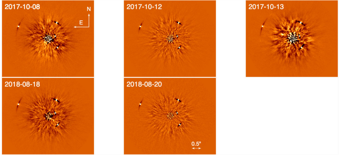
Figure 3. Full sequence reduced images for data taken in October 2017 and August 2018. Data were processed using the VIP PCA pipeline (Gomez Gonzalez et al. 2017), removing 25 principal component modes. All four planets are easily detected; the image scale runs from -10 to 10 ADU and has been adjusted to highlight the residual speckle noise remaining after subtraction of the principal modes.
