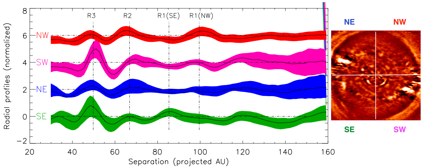
Fig. B.3. Radial profiles of the KLIP IRDIS-H2H3 deprojected image as measured in four quadrants shown in the right panel (red : north-west, magenta : south-west, blue : north-east and green : south-east). Black lines stand for averaged profile and the colour shaded areas indicate the azimuthal dispersion. All profiles are normalized and vertically shifted for the sake of clarity
