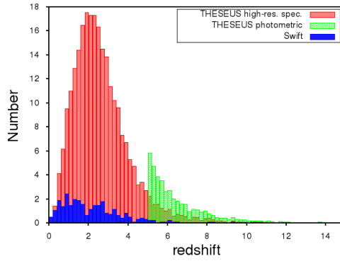
Fig. 4. The redshift distribution of THESEUS GRBs during a 5 yr mission lifetime compared to the actual distribution of Swift GRBs (blue) during the same period. GRBs with a photometric redshift are in green, and those with a spectroscopic redshift are in red.
