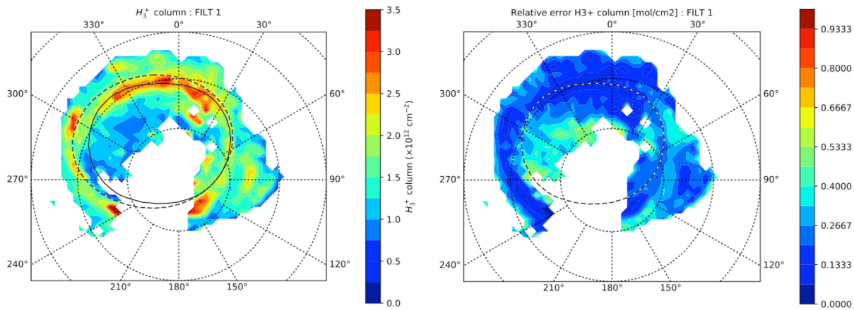
Figure 4. H_3^+ column density (left panel) and error on its retrieval (right panel). The continuous curve oval is from VIP4 model [Connerney et al. , 1998]; the dashed curve oval it the statistical one from ground-based observations [Bagenal et al. , 2014]. Latitudes are spaced by 10 degrees
