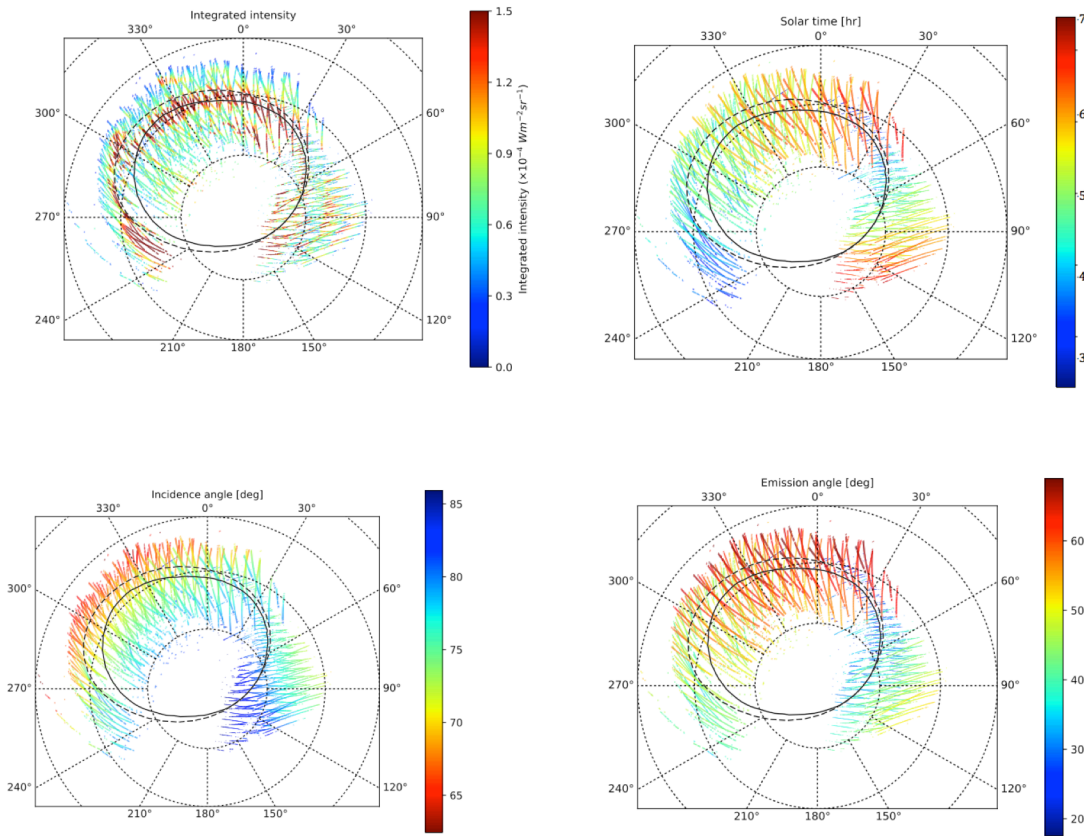
Figure 2. Southern aurora observational parameters: \text{H}_3^+ auroral emissions integrated in the range 3.35 to 3.75 \mu\text{m} (upper left); Time of the Jovian day upper right); Solar Zenith Angle (SZA) (lower left); and Emission Zenith Angle (angular direction of the spacecraft in respect the emitting area) (lower right). Latitudes are spaced by 10 degrees. The continuous curve oval is from VIP4 model [Connerney et al. , 1998]; the dashed curve oval it the statistical one from ground-based observations [Bagenal et al. , 2014].
