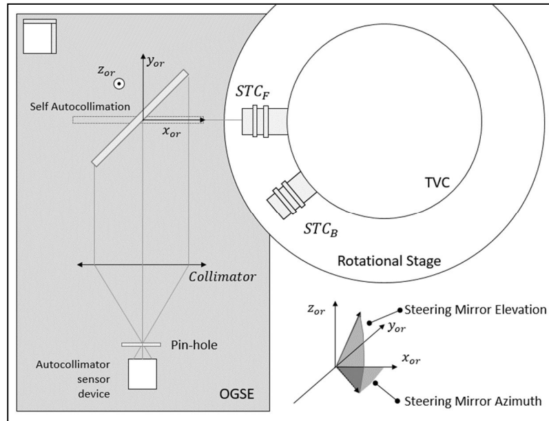
Figure 2. OGSE schematic diagram and reference system definition.
