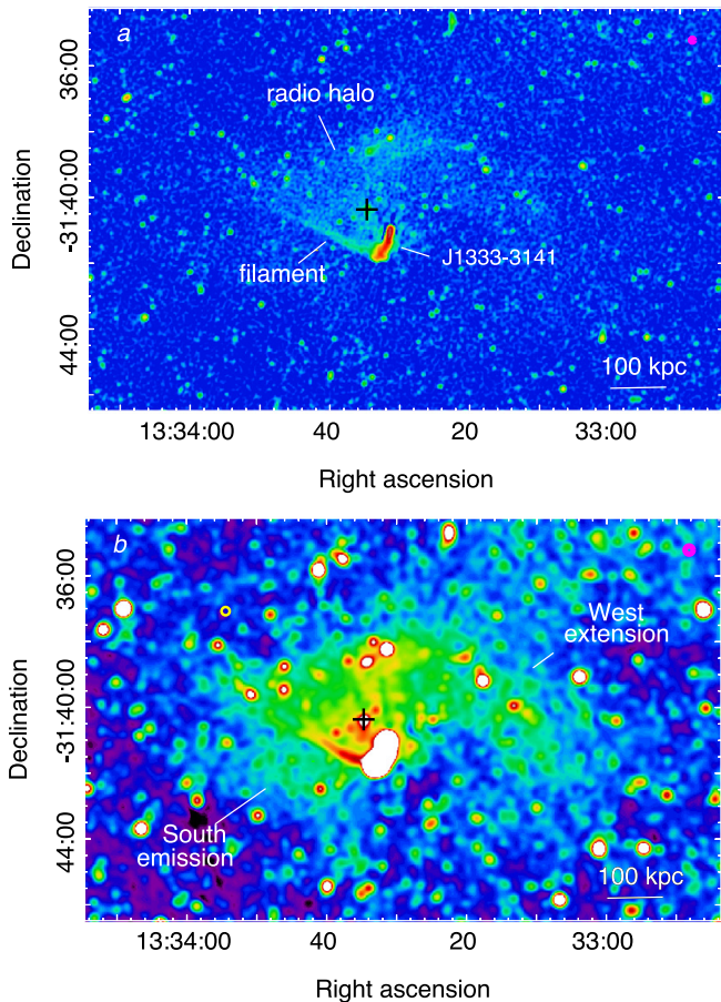
Figure 1. MeerKAT 1284 MHz images with an angular resolution of 6''4 \times 6''0 , in position angle (a) 146^\circ and (b) 15^\circ . The beam size (FWHM) is shown by a magenta circle in the upper right corner of each panel. The rms noise is 1\sigma = 6 \mu\text{Jy beam}^{-1} and 1\sigma = 9 \mu\text{Jy beam}^{-1} , respectively. The black plus sign marks the position of the BCG.
