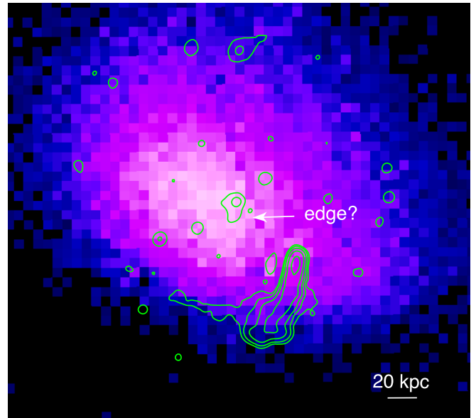
Figure 11. The core of A3562. This is the same XMM X-ray image as in Figure 8(c), with the colors chosen to emphasize the possible X-ray brightness edge near the central galaxy. Radio contours are as in Figure 3.
