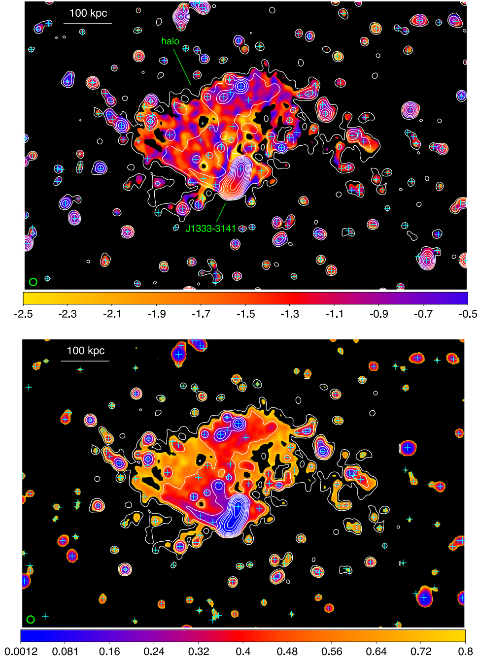
Figure 4. Color-scale images of the MeerKAT in-band (1070–1498 MHz) spectral index distribution in the head–tail source J1333–3141 and radio halo at a resolution of 15'' (top) and corresponding uncertainty map (bottom). Color bars are the spectral index (top) and spectral index error (bottom). In both panels, the contours from the full-band image at matching resolution (Figure 1(b)) are overlaid on the color map. Contours start at 5\sigma = 45 \mu\text{Jy beam}^{-1} and scale by a factor of 2. Cyan plus signs mark the position of the discrete radio sources identified by the PyBDSF source finding on the full-band, high-resolution image (Figure 1(a)). The beam size is shown by the green circle in the lower left corner of each panel.
