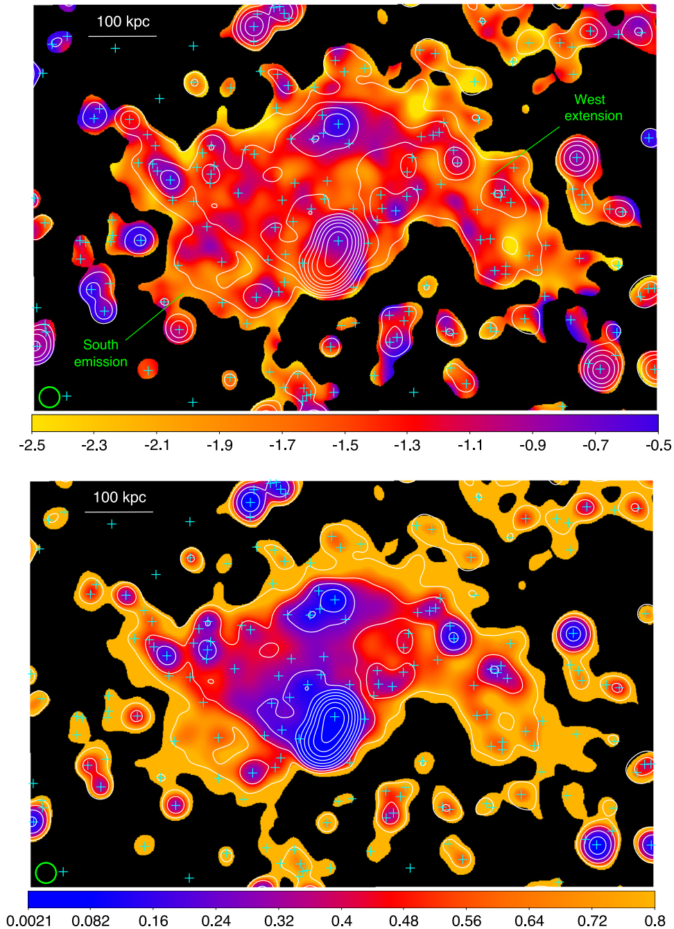
Figure 5. Color-scale images of the MeerKAT in-band (1070–1498 MHz) spectral index image at a resolution of 30'' (top) and corresponding uncertainty map (bottom). Color bars are the spectral index (top) and spectral index error (bottom). In both panels, the contours from the full-band image at matching resolution are overlaid on the color map. Contours start at 5\sigma = 75 \mu\text{Jy beam}^{-1} and scale by a factor of 2. Cyan plus signs mark the position of the discrete radio sources identified by the PyBDSF source finding on the full-band, high-resolution image (Figure 1(a)). The beam size is shown by the green circle in the lower left corner of each panel.
