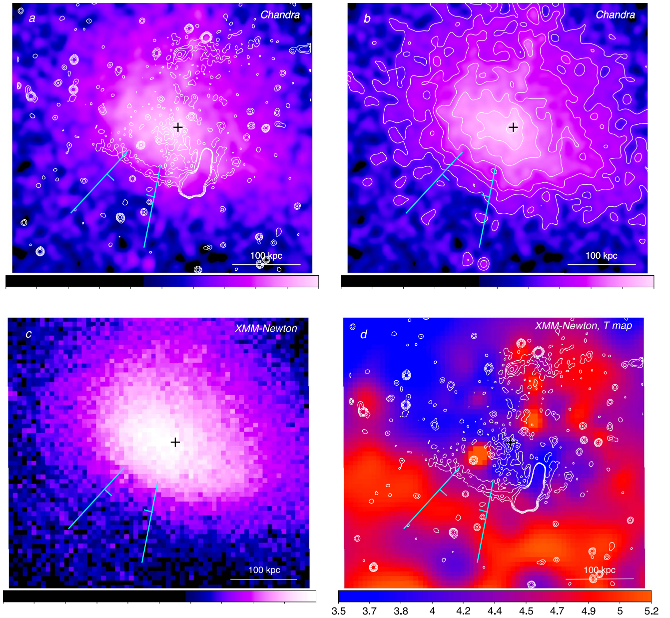
Figure 8. (a) Chandra image in the 0.5–4 keV band, smoothed with a 5'' Gaussian. The image is background subtracted and divided by the exposure map. Radio contours from Figure 1(a) are overlaid at 24 ( 4\sigma ), 48 , 96 and 192 \mu\text{Jy beam}^{-1} . (b) Chandra 0.5–4 keV image as in panel (a), with contours of the core X-ray emission overlaid, spaced by a factor of \sqrt{2} . (c) XMM-Newton image in the 0.5–2.5 keV band (V22). (d) XMM-Newton temperature map (V22). In all panels, the black plus sign marks the position of the BCG. The cyan sector is used for the radial profiles (Figure 9); short ticks show the position of a cold front. Color bars show the X-ray surface brightness in arbitrary units (panels (a), (b), and (c)) and temperature in keV (panel (d)).
