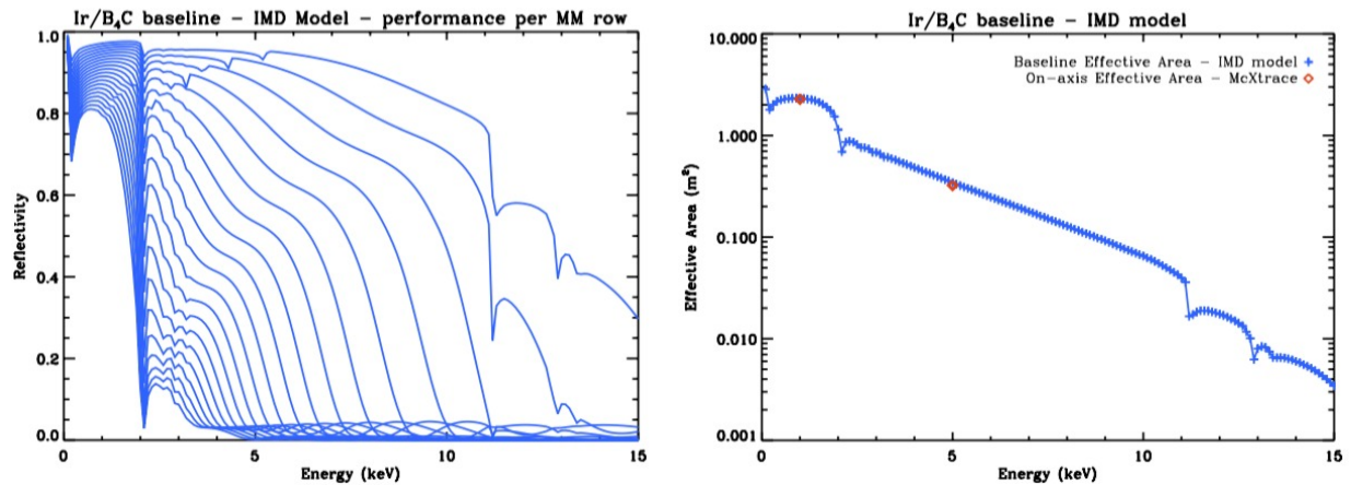
Figure 7. Left: Coating reflectivity theoretical model generated using IMD considering the incident grazing angles at the centre of the mirror module rows. Right: On-axis effective area theoretical model along with the simulated effective areas (red) at 1 keV and 5 keV.
