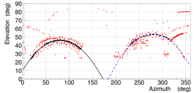
Figure 8. Transient candidates from 2020 April 10/11 data overplotted with second-order polynomials fitted to two paths. These parabolas were later used in excising RFI from aircraft moving along these routes.
