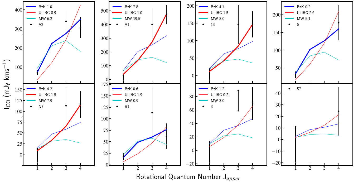
Figure 6. CO SLEDs of eight cluster galaxies detected in CO[4–3]. The legends show the reduced \chi^2 value for the fits of the observed galaxy CO SLED with the three excitation models: BzK, ULIRG/SB, and MW. The SLEDs of some galaxies are best-fit by a BzK excitation model, and some are best-fit by a ULIRG/starburst-like model. The preferred template for each galaxy is plot with a thicker line, where possible. We do not draw any conclusions about the gas excitation of galaxies ID 3 and S7, due to the limited data available. A least-squared analysis was used for the fitting, and 2\sigma flux upper limits are shown.
