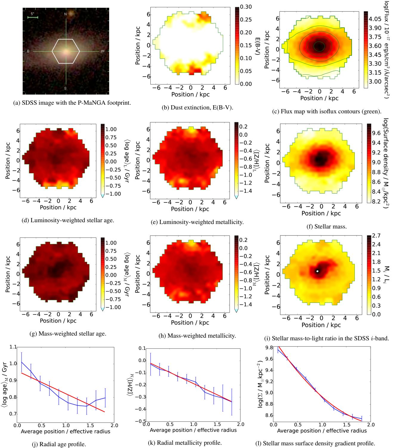
Figure 5. Group \alpha , galaxy p9-19B as in table 2. Stellar population maps and profiles analyzed using MILES-based models with their full parameter range. The radial profiles are over-plotted in red with a linear fit to the data, in the age and metallicity profiles to show the derived gradient, and a quadratic fit in the stellar mass density profile in order to guide the eye. We use a pixel-to-pixel Gaussian filter to smooth the maps for ease of visualisation, but use a 0.5 sigma kernel in order to retain small-scale features. This galaxy has been observed with good observational conditions with a MaNGA-like exposure time and dithering, and is selected in the MaNGA primary sample. Therefore out of the P-MaNGA dataset, these observations are the most similar to the expected output of the MaNGA primary sample.
