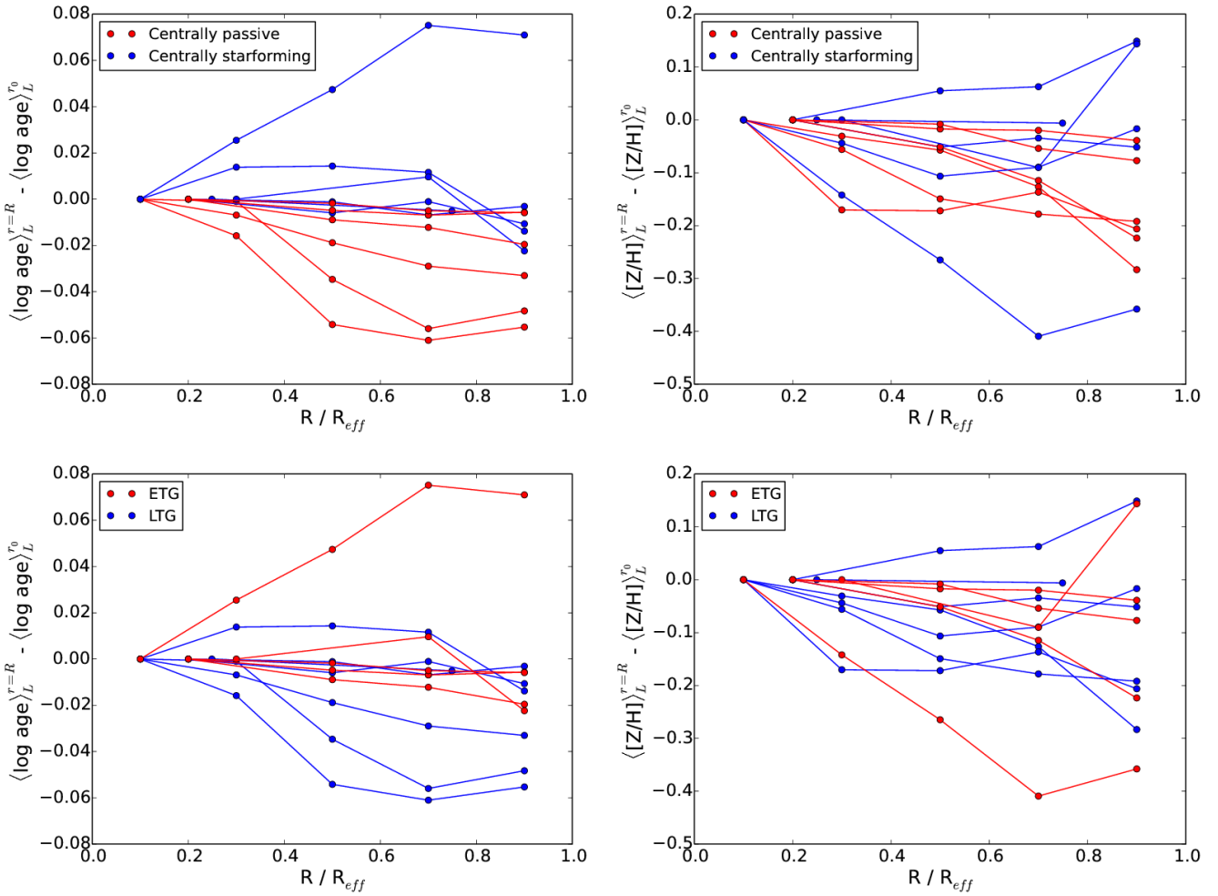
Figure 19. Light-weighted age and metallicity gradients up to 1 effective radius, plotted as the change in age / metallicity from the first elliptical annular bin, where each line represents the profile from a P-MaNGA galaxy. In the upper panels we use the classifications of centrally quiescent/passive or centrally starforming as described in Li et al. (2015). In the lower panels we use the morphological classifications in this paper (as in Table 2). Bins are 0.2 effective radius in size to match Li et al. (2015) as much as possible, however we impose a condition that each bin must contain at least 10 pixels from the corresponding data cube. If this condition is not met we sample at wider bins until the criterion is met, in order to ensure a reliable mean age or metallicity at each point.
