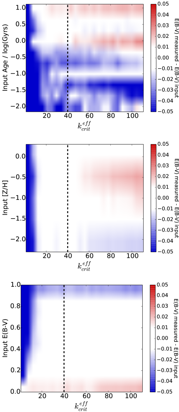
Figure 4. Tests showing the recovery of dust values (in terms of difference between E(B-V) recovered to input E(B-V) ) from mock galaxy spectra from MILES-based models as a function of the number of large-scale modes excluded in the fit. The number of modes excluded is described by an effective k_{crit}^{eff} parameter (in equation 3). The three plots show recovery of dust as a function of the following input properties: age, metallicity and extinction respectively. In each case, the values plotted are marginalised over the other two input properties. The black dashed line marks the value of k_{crit}^{eff} used in this paper for the analysis of P-MaNGA galaxies. Each mock galaxy spectra is constructed by perturbing each flux point of an input model SSP by a Gaussian probability distribution on each point, assuming a flat signal to noise of 10 across the whole wavelength range. A signal-to-noise of ten was chosen as it is typical of the outer regions of most P-MaNGA galaxies.
