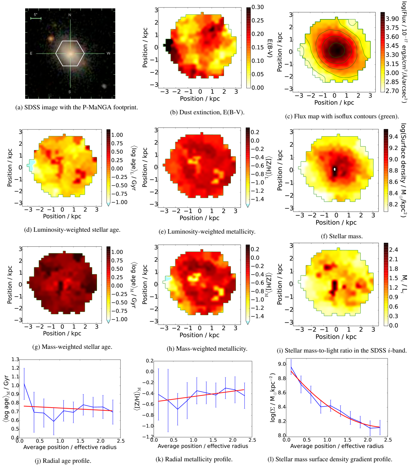
Figure 21. Group \alpha , galaxy p9-19E as in table 2. Stellar population maps and profiles analyzed using MILES-based models with their full parameter range, as described in detail in Figure 5. This galaxy has been observed under good observational conditions with MaNGA-like exposure time and dithering, but covers a larger radial extent than would be targeted in the MaNGA primary sample. However it is selected by the MaNGA secondary sample.
