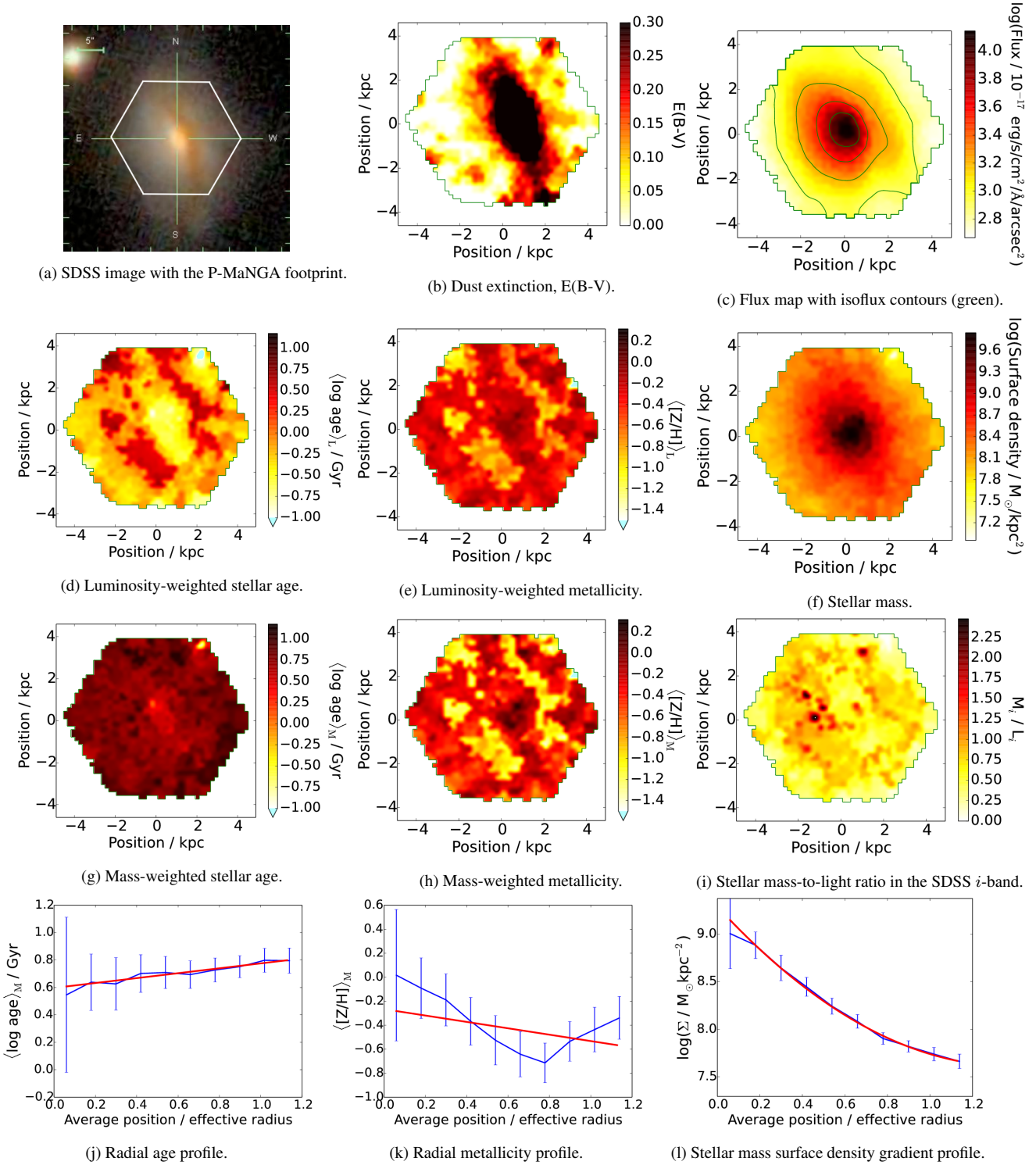
Figure 6. Group \beta , galaxy p9-61A as in table 2. Stellar population maps and profiles analyzed using MILES-based models with their full parameter range, as described in detail in Figure 5. Observed under the same setup as galaxy p9-19B (Figure 5), except with a N 61 IFU, and observed to a higher spatial resolution than would be targeted for the MaNGA sample.
