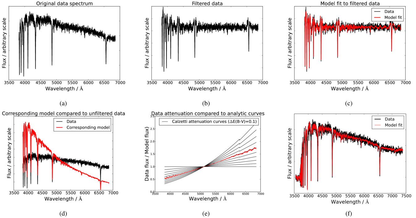
Figure 3. Example of fitting a spectrum for dust using a high-pass filter. Starting top-left and moving horizontally, the panels describe each stage of the filter and fitting process. Panel a) shows the input model spectrum corresponding to a 30 Myr, [Z/H] = 0 SSP with a signal-to-noise applied at each flux point of 50. Panel b) shows that data processed through a high-pass filter that removes large-scale features such as continuum shape and dust extinction. Panel c) shows the fit to the filtered spectrum using models that are filtered in the same way. All models used to make this fit have E(B-V) = 0 since we would be removing the effect of dust attenuation on the models anyway. Using the same parameters determined through the fit in c), panel d) shows the corresponding parameters in the unfiltered model case. We expect to see a systematic tilt between the data and models, corresponding to a dust attenuation curve. In panel e) we find the best value for E(B-V) by calculating the [data / model] spectrum and fitting this to a range of attenuation curves across the whole spectrum. In practice we used \Delta E(B-V) of 0.01, but intervals of 0.10 are shown here for clarity. The best fitting E(B-V) for this case is 0.50, exactly matching our input value of 0.50. Lastly we use the value of E(B-V) obtained to re-fit the original data using unfiltered attenuated models. Panel f) shows the final fit obtained across the whole wavelength range.
