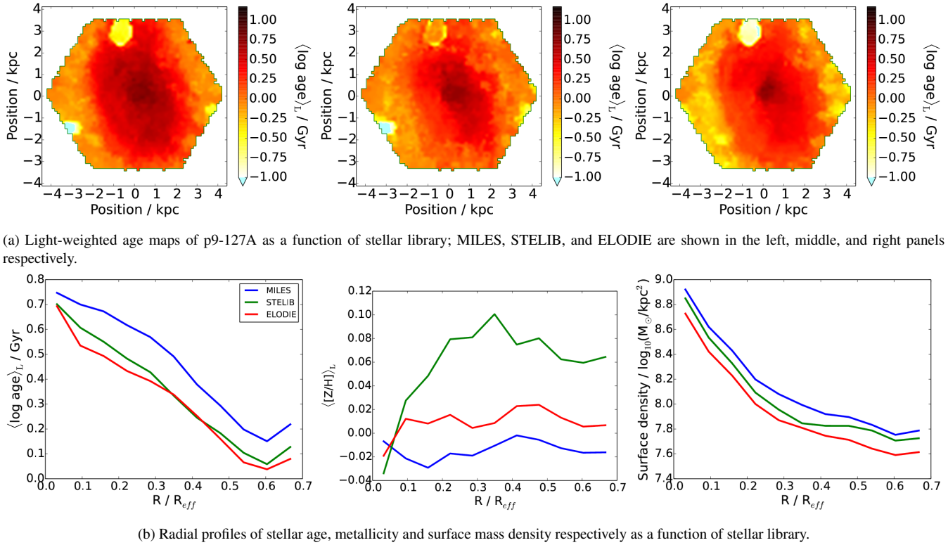
Figure 15. The effect on galaxy properties of the stellar library input in the stellar population model. In all cases, models were fit with identical stellar population parameter grids (see section 3.1). Maps are composed of Voronoi binned cells of properties, corresponding to binned spectra that cover enough sky area such that the median signal-to-noise at any given cell is as close as possible to 5. Typically this means that the outer Voronoi cells of the galaxy cover a more extended area than the inner cells. The radial properties are computed from spectra summed in annuli that have radial extent that approximately scales logarithmically, in order to give the surface mass density (right-hand side) profiles.
