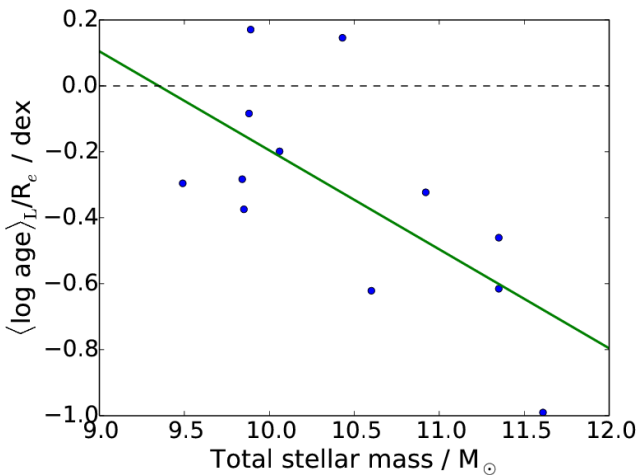
Figure 11. A scatterplot showing the relation between photometric stellar masses and \langle \log \text{age} \rangle_L , as derived in this paper, for the late-type galaxies in the P-MaNGA sample as listed in Table 2. This relation is plotted in order to compare to the conclusions of González Delgado et al. (2014) (see text). In dashed black we show zero gradient line, and in green we show a linear regression line.
