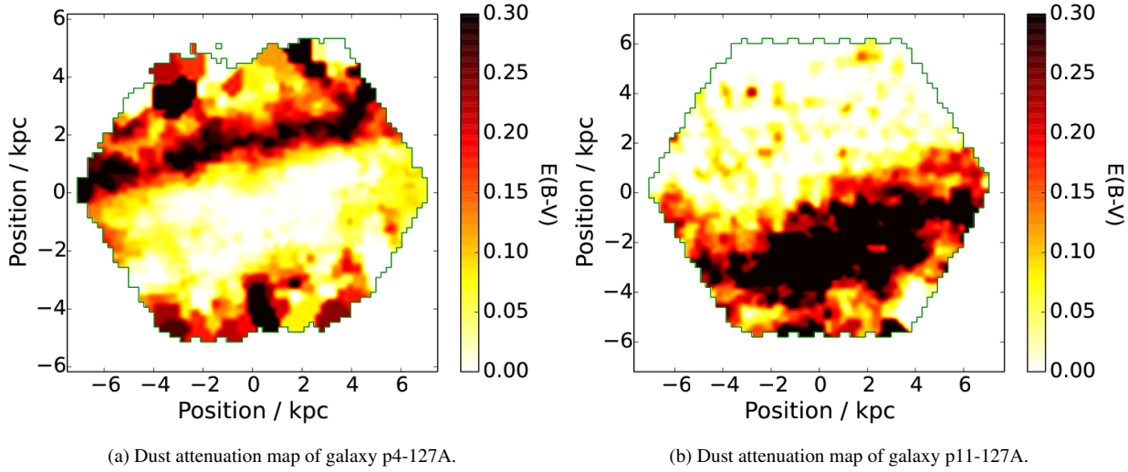
Figure 8. Group \delta galaxies p4-127A and p11-127A as in table 2. These two galaxies have very clear dust lanes that show evidence of more recent star formation than their surroundings. Both of these galaxies have been observed under poorer conditions and lower exposures and dithering setup than expected for MaNGA, although p4-127A has been observed under worse conditions and setup than p11-127A, translating to a more speckled appearance in its maps.
