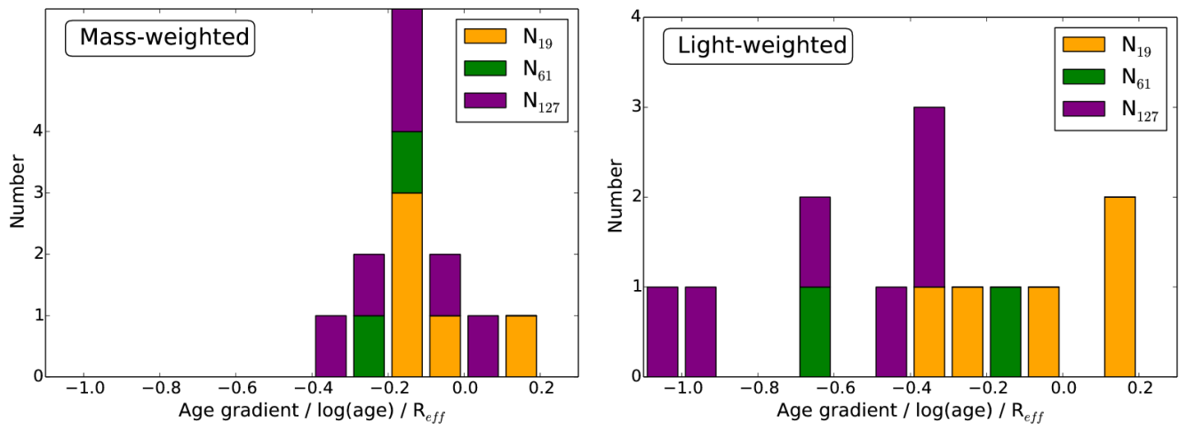
Figure 12. Histograms of age gradients as in Figure 10, selecting only the late-type galaxies in the sample, but as a function of IFU size. In the left panel we show mass-weighted age gradients as in the other profile and gradient Figures in this paper. In the right panel we show light-weighted age gradients since these will trace bright stellar populations, and thus are important for testing the effect of beam smearing.
