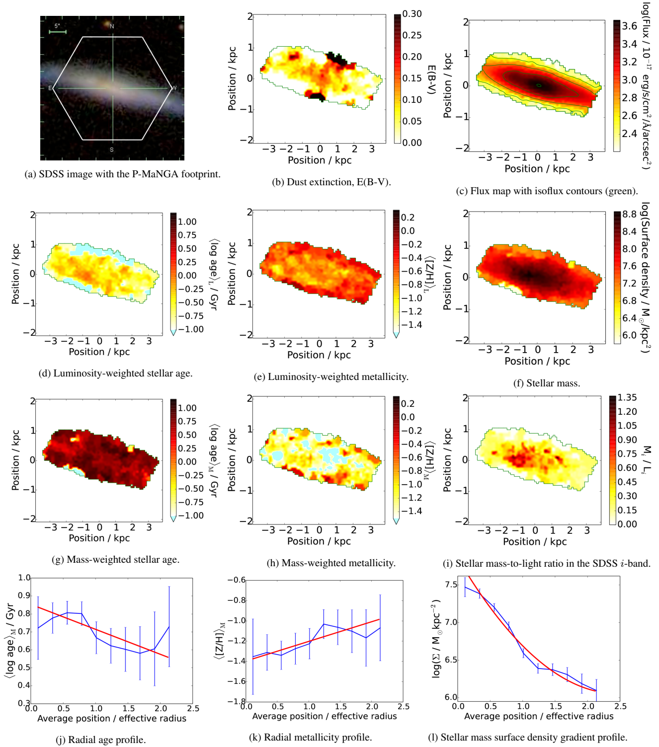
Figure 22. Group \alpha , galaxy p9-127B as in table 2. Stellar population maps and profiles analyzed using MILES-based models with their full parameter range, as described in detail in Figure 5. This galaxy has been observed under good observational conditions with MaNGA-like exposure time and dithering, but covers a larger radial extent than would be targeted in the MaNGA primary sample, like galaxy p9-19E (Figure 21), and is selected by the MaNGA secondary sample.
