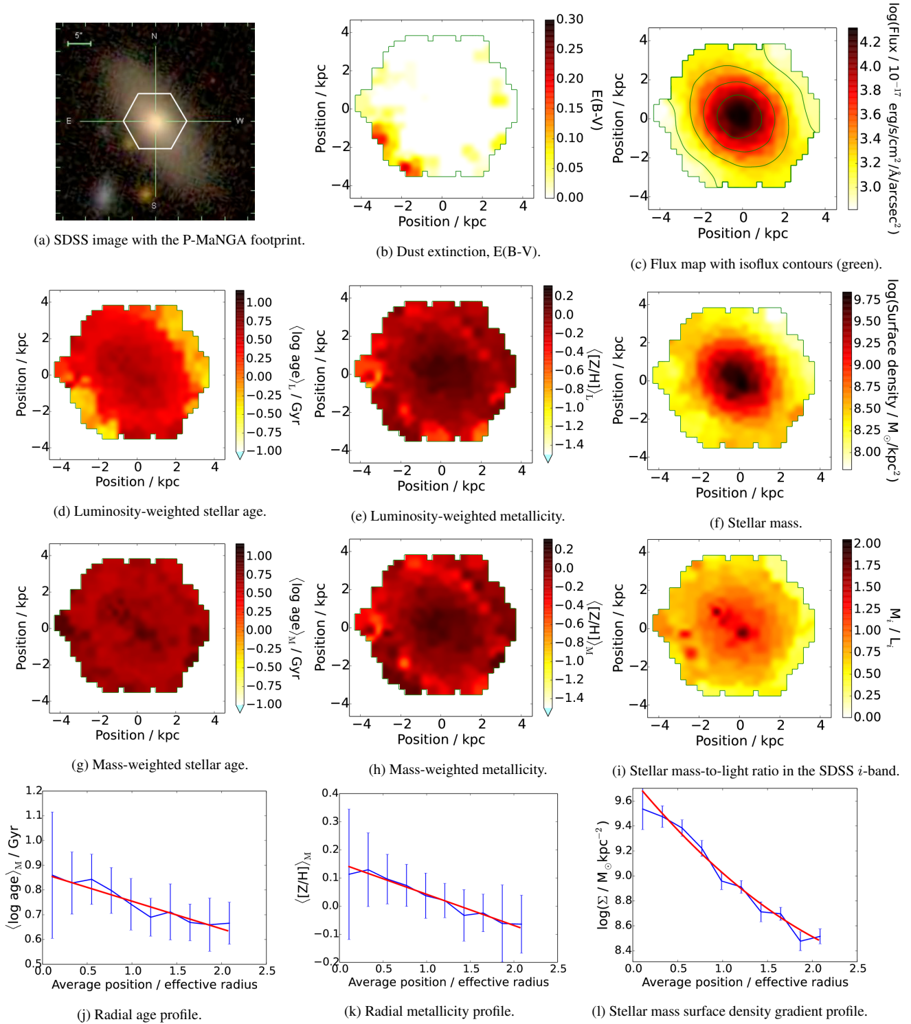
Figure 20. Group \alpha , galaxy p9-19D as in table 2. Stellar population maps and profiles analyzed using MILES-based models with their full parameter range, as described in detail in Figure 5. This galaxy, like p9-19B in Figure 5, has been observed with good observational conditions with a MaNGA-like exposure time and dithering, and is selected in the MaNGA primary sample. Therefore out of the P-MaNGA dataset, these observations are the most similar to the expected output of the MaNGA primary sample.
