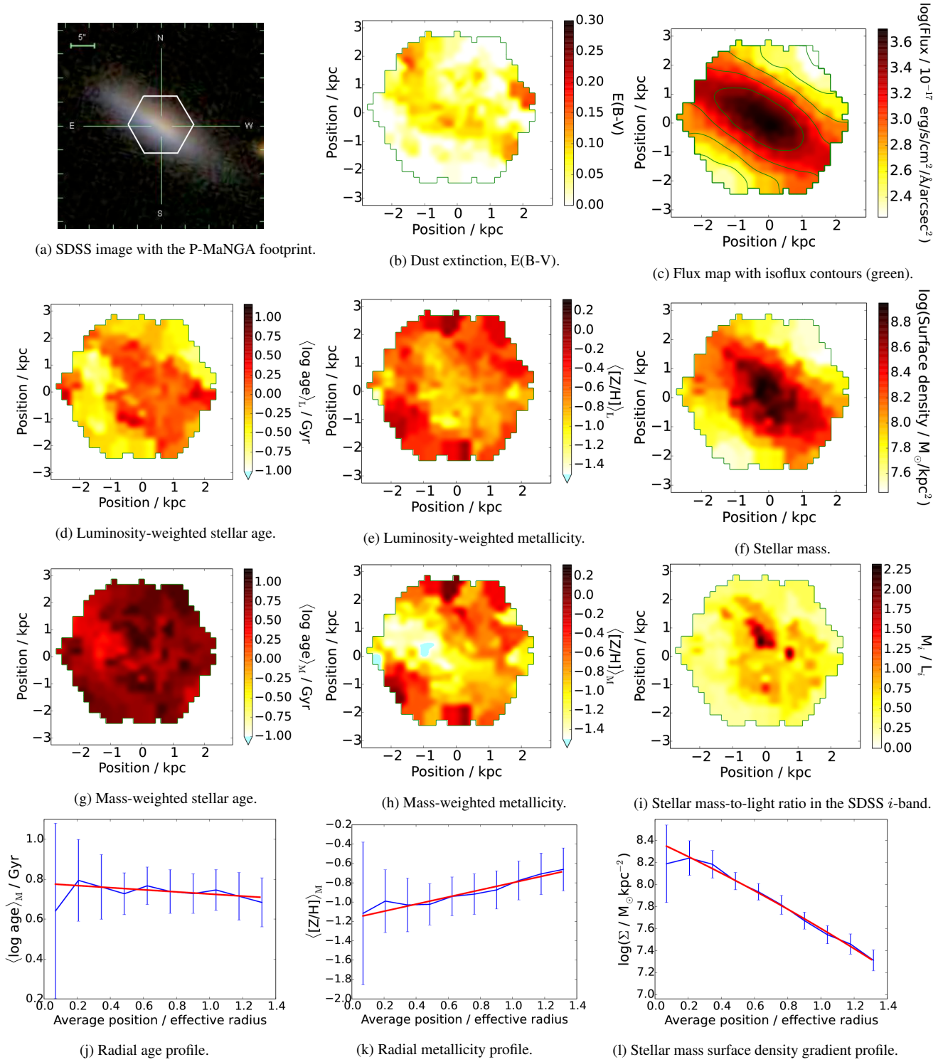
Figure 24. Group \gamma , galaxy p4-19B as in table 2. Stellar population maps and profiles analyzed using MILES-based models with their full parameter range, as described in detail in Figure 5. This galaxy has been observed under poorer conditions and a lower exposure and dithering setup than expected for MaNGA. Unlike galaxy p4-19C (Figure 7), we resolve a more complex stellar population structure that reflects the asymmetric colour distribution seen in the SDSS image.
