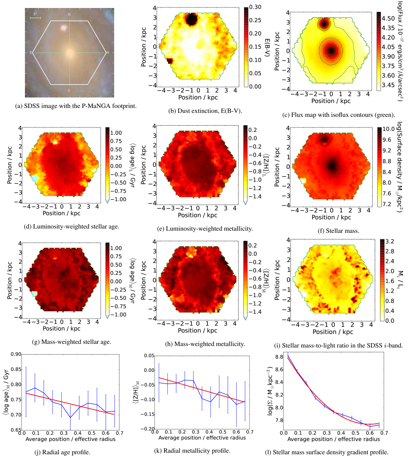
Figure 23. Group \beta , galaxy p9-127A as in table 2. Stellar population maps and profiles analyzed using MILES-based models with their full parameter range, as described in detail in Figure 5. This galaxy is taken under MaNGA-like observational conditions and setup, but is not targeted in the main MaNGA samples due to its low redshift, and therefore radial coverage by MaNGA IFUs. Hence this galaxy is observed with a higher amount of structural detail than we should expect to observe with MaNGA.
