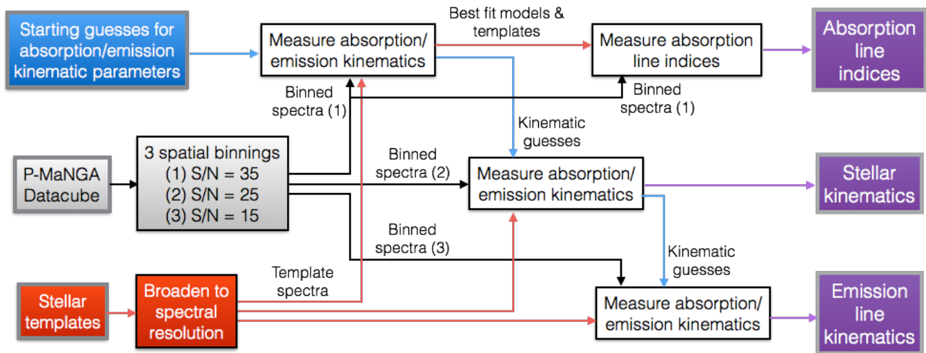
Figure 1. Summary of the processes of the Prototype Data Analysis Pipeline (PDAP), used to recover the physical parameters used as input in this work in addition to the P-MaNGA datacubes. P-MaNGA datacubes are binned in three spatial schemes according to the signal-to-noise requirements of the properties extracted from the kinematic fits. Each of the processes are described in section 2.1. Each kinematic fit also outputs improved starting kinematic guesses for the next spatial bin.
