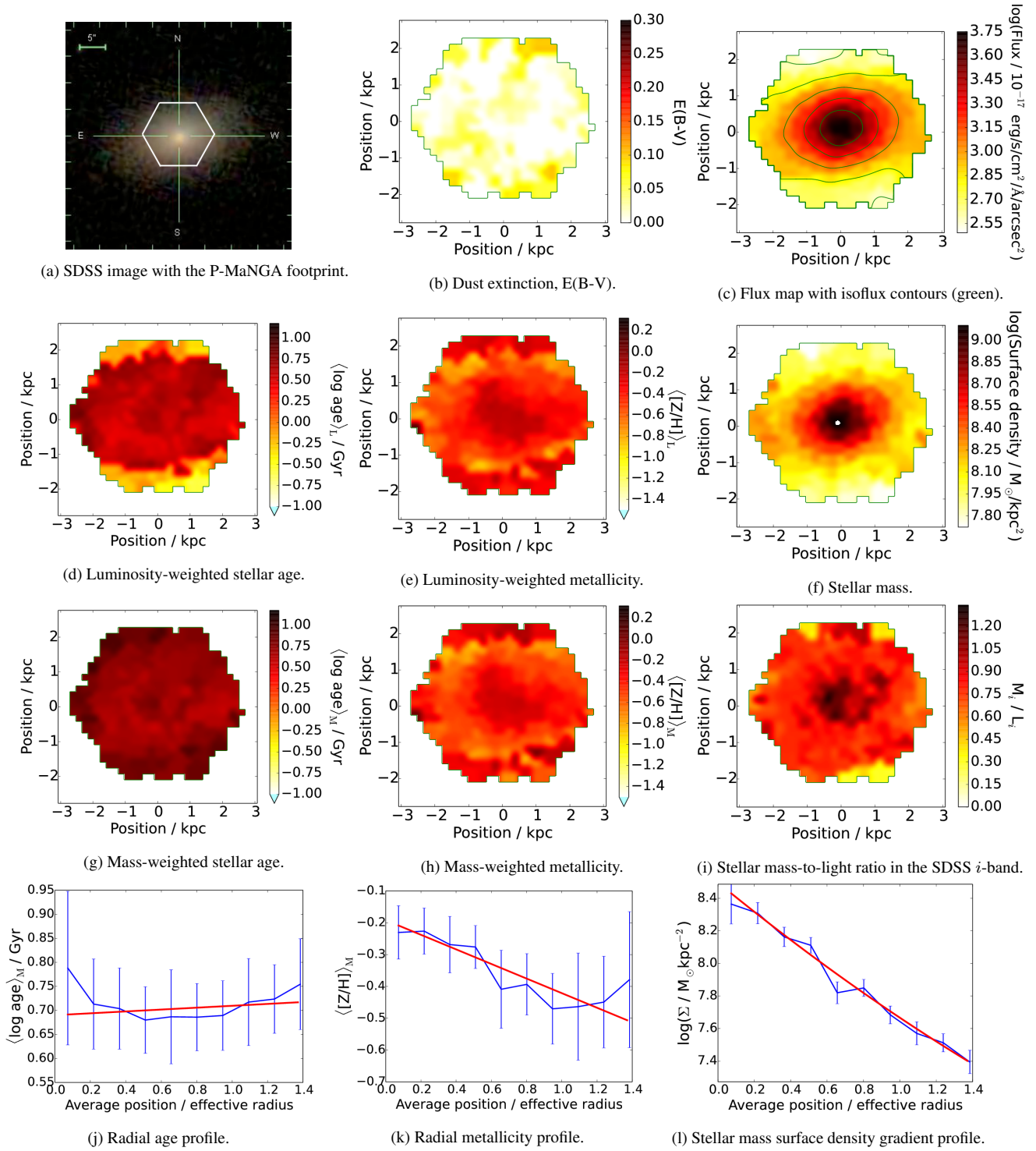
Figure 7. Group \gamma , galaxy p4-19C as in table 2. Stellar population maps and profiles analyzed using MILES-based models with their full parameter range, as described in detail in Figure 5. This galaxy has been observed under poorer conditions and a lower exposure and dithering setup than expected for MaNGA. Nonetheless, we recover a simple and smooth stellar population structure with negative age and metallicity gradients.
