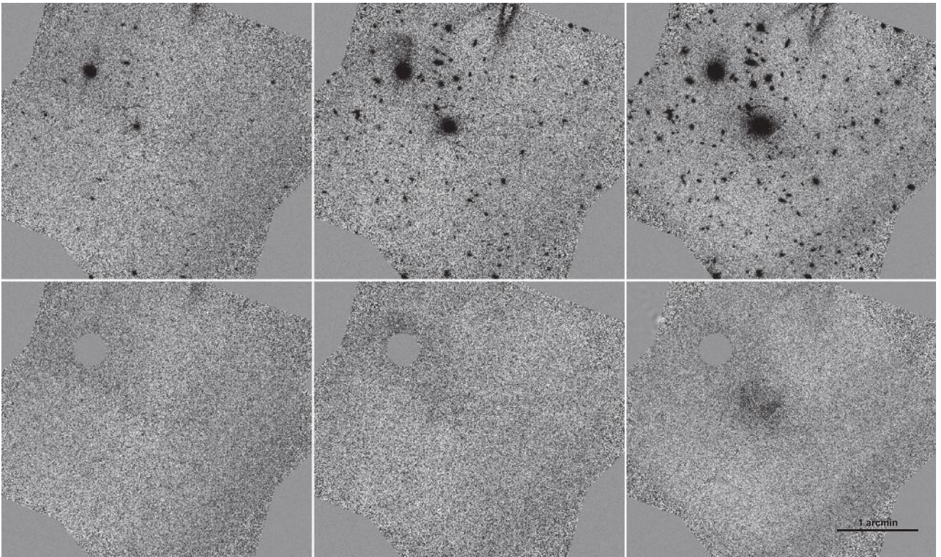
Figure 5. Original images of the relaxed cluster MS 2137 (top) and ICL+background maps provided by CICLE (bottom) in the F435W, F625W, and F814W filters (from left to right). The scale of the original and ICL+background images is the same for each filter.
