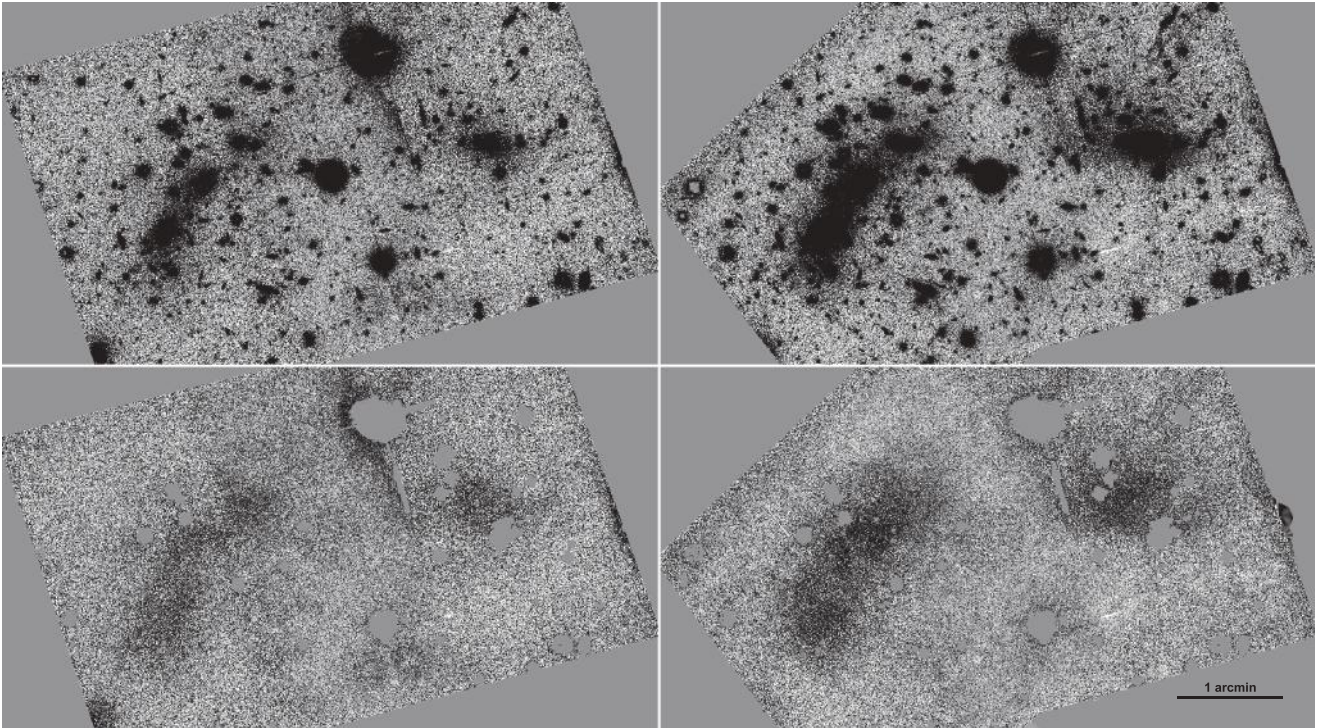
Figure 13. Original images of the unrelaxed Bullet cluster (top) and ICL+background maps provided by CICLE (bottom) in the F606W and F814W filters (from left to right). The scale of the original and ICL+background images is the same for each filter.
