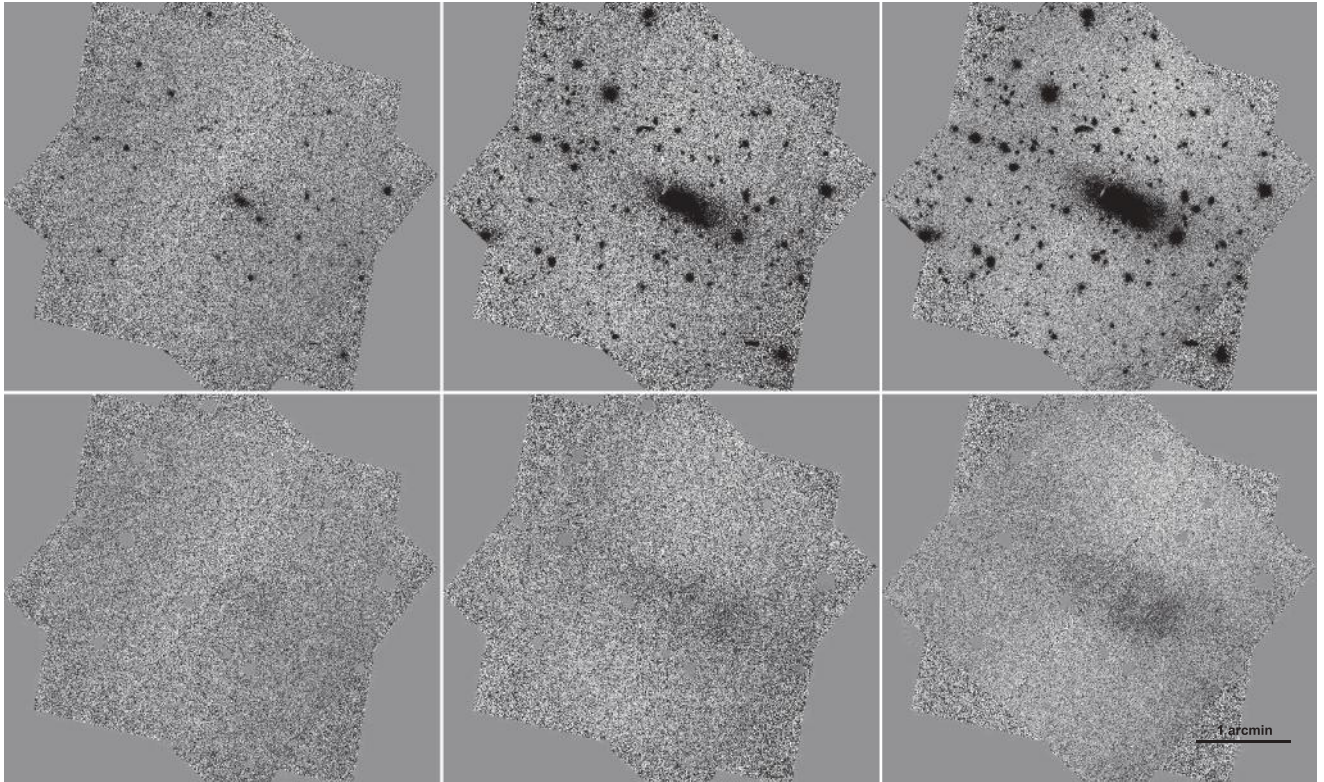
Figure 7. Original images of the relaxed cluster RXJ 2129 (top) and ICL+background maps provided by CICLE (bottom) in the F435W, F606W, and F814W filters (from left to right). The scale of the original and ICL+background images is the same for each filter.
