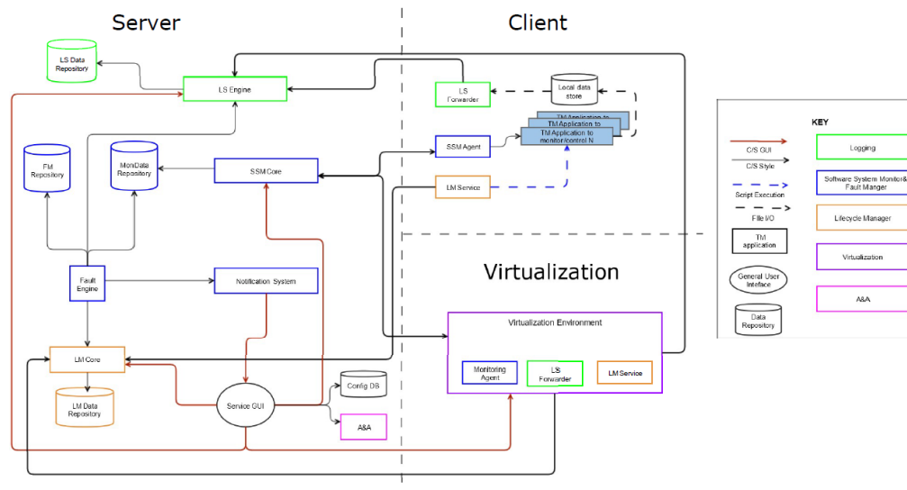
Figure 5: Runtime view.
