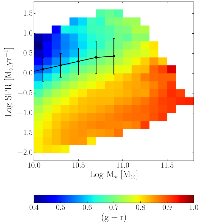
Figure 4. Distribution of galaxies in the \log(\text{SFR}) – \log(M_*) plane colour-coded as a function of the mean g-r colour in bin of SFR and stellar mass. The mode of the MS at different stellar mass bins is overplotted (connected points). The error bars show the dispersion of the relation around the mode.
