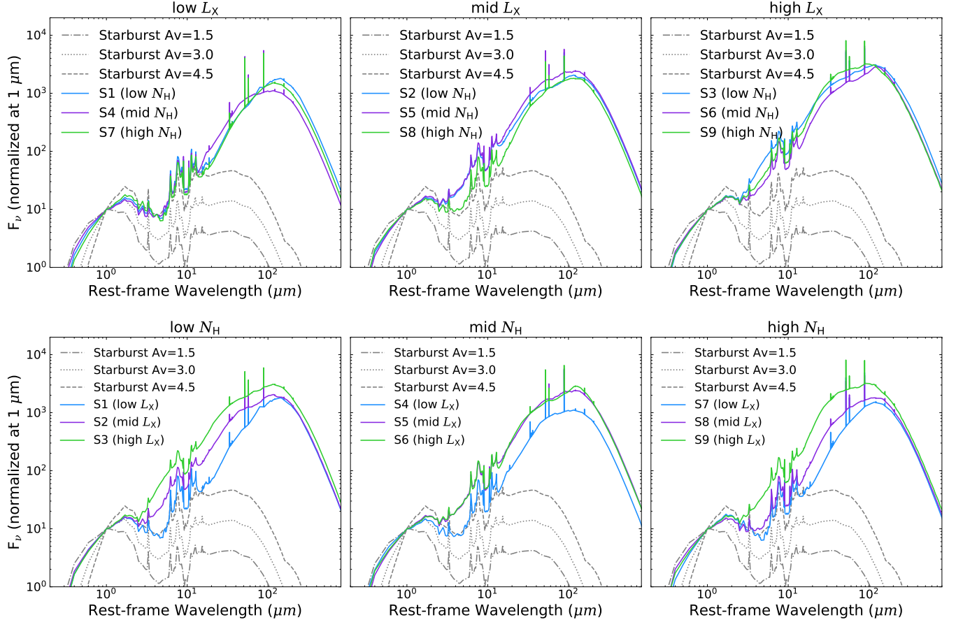
Figure 5. Composite (stellar + AGN) SEDs for highly obscured AGNs in different L_X and N_H bins (i.e., S1 – S9) defined in Figure 4. Top (Bottom): Comparison of SED shapes at a given L_X ( N_H ) bin. Each gray curve shows the M82 galaxy template that is attenuated using a specified extinction value (without adding the dust re-radiation component in FIR).
