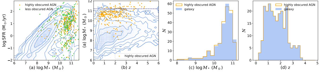
Figure 9. (a) SFR vs. M_* relation for our sample of highly obscured and less obscured AGNs compared to that of non-active galaxies (blue contours) in Santini et al. (2015). (b) M_* vs. z for highly obscured AGNs relative to non-active galaxies. The horizontal dashed line marks out stellar mass cut at \log M_*/M_\odot = 11.2 . (c, d) M_* and z distributions for typical randomly-selected highly obscured AGNs and their corresponding control galaxies from our sampling procedure.
