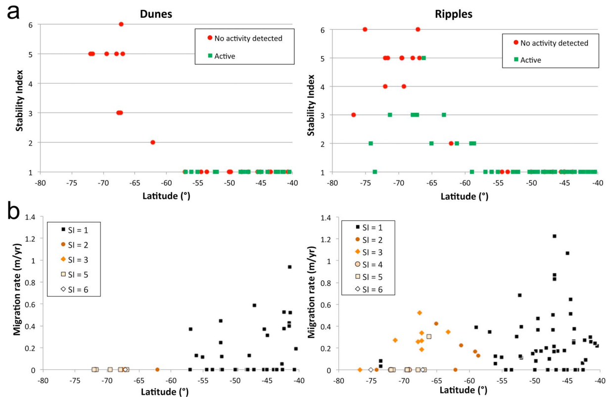
Figure 6. (a) Dune field stability index with latitude, marked by (left) dune and (right) ripple mobility. Note the near lack of mobility for ripples in SI \geq 4 dune fields and for dunes in SI \geq 2 dune fields. (b) Average (left) dune and (right) ripple migration rates with latitude, colored by dune field stability index. Bedforms that show no evidence of activity (inactive) and active bedforms with ambiguous or unquantified movement plot with a migration rate of 0. Note the decrease in migration rates with higher SI.
