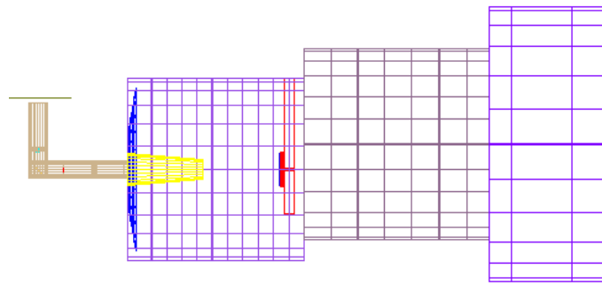
Figure 14 Displaced EB (exaggerated)
