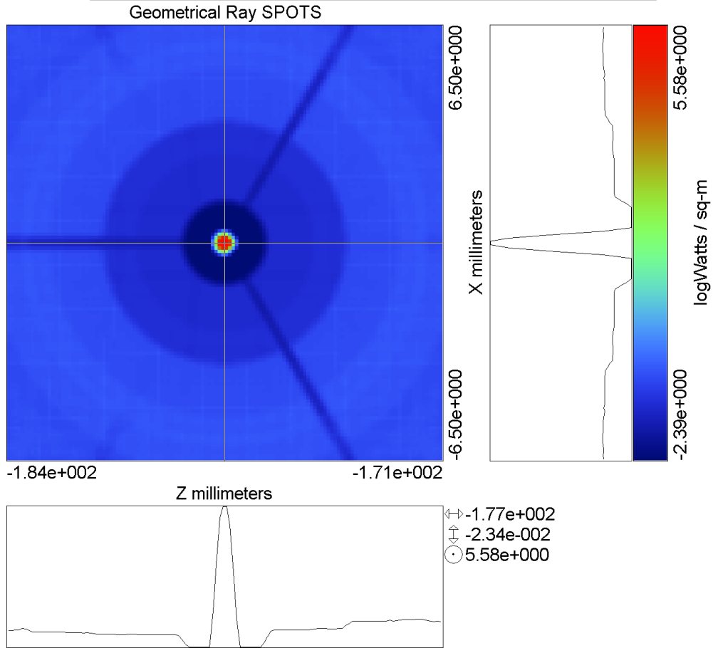
Figure 33: On Axis Image and ghosts. Scale is logarithmic and values are relative to source of 1 W/mm^2
