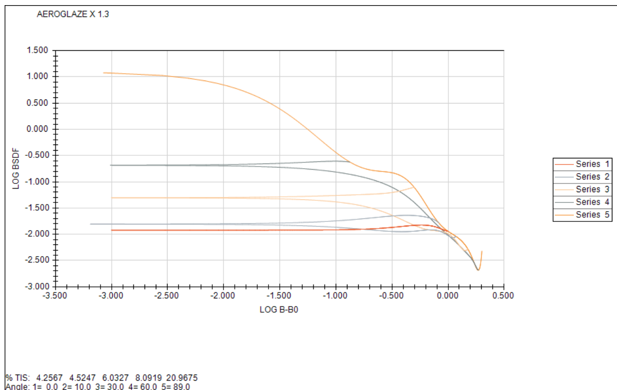
Figure 10: ASAP Aeroglaze 306 model BRDF, 1.3 Factor
