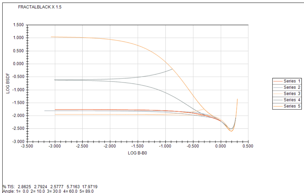
Figure 11: Fractal Black BRDF, binomial model, 1.5 factor.
