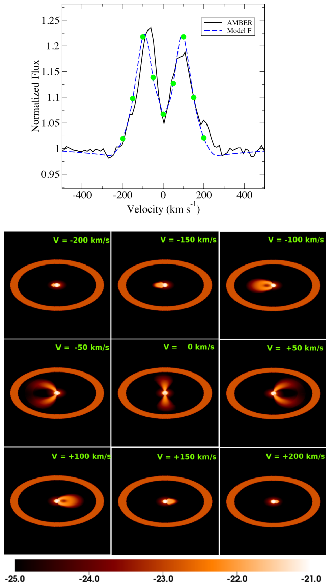
Figure 7. Upper panel: the model \text{Br}\gamma profile (dash) computed at i = 55^\circ with the magnetosphere and disc wind (Model F in Table 6) is compared with the AMBER observation (solid). The velocity channels at which the emission maps (lower panel) are computed are indicated by filled circles. The corresponding emission maps (in logarithmic scale and in arbitrary units) at nine different velocity channels are shown in the lower panel. The image sizes are 1.89 \times 1.89 \text{ au}^2 or 5.94 \times 5.94 \text{ mas}^2 , assuming the object is at 318 pc (VL07). The wavelength/velocity dependent images shown here are used to compute the interferometric quantities such as visibilities, differential phases and closure phases as a function of wavelength/velocity.
