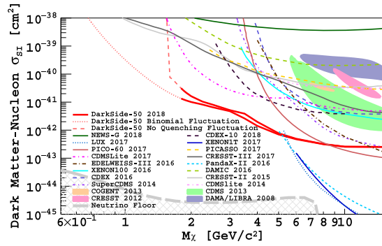
FIG. 8. Ninety percent upper limits on spin-independent DM-nucleon cross sections from DarkSide-50 in the range above 1.8 \text{ GeV}/c^2 . See the text for additional details.
