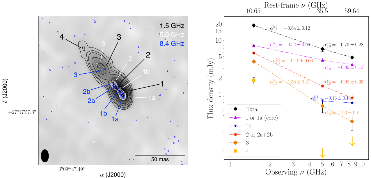
Fig. 2: Left : Overlay of the 1.5 (black contours), 5 (white contours) and 8.4 GHz (blue contours) emission of PSO J0309+27. The greyscale map is the 1.5 GHz self-calibrated image, and its restoring beam is shown on the bottom left corner; north is up, east is left. The phased referenced absolute position of component 1a is 03^{\text{h}}09^{\text{m}}47.4862^{\text{s}}, +27^{\circ}17'57.3165'' . Right : Radio spectrum of all the sub-components of PSO J0309+27 spatially resolved by the multi-frequency VLBI observations presented here. We indicate with the arrows the 3\sigma detection limit for sub-component 4 at 5 and 8.4 GHz, estimated as three times the flux density within the same area of the 1.5 GHz detection of that sub-component.
