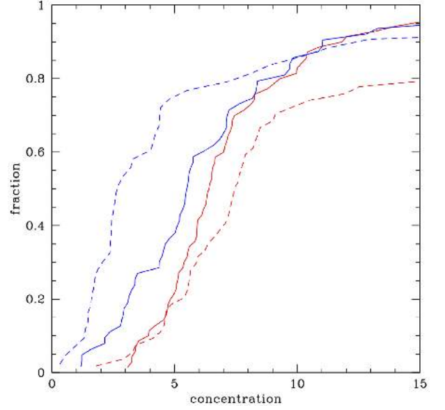
Figure 9. Cumulative distribution of concentration values for each cluster sub-sample (see text for details). XXL N > 15 and N < 15 are displayed as solid and dashed red lines. CAMIRA high-flux matched and unmatched clusters are displayed as solid and dashed blue lines. For reference, a flat surface brightness profile will result in a concentration value of unity.
