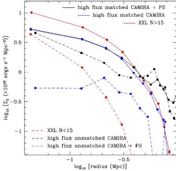
Figure 8. XSB distributions for each cluster sub-sample. Profiles are displayed for XXL N > 15 (solid red line) and N < 15 (dashed red line) together with high flux CAMIRA matched (solid blue line) and unmatched (dashed blue line). We additionally plot the surface brightness profiles for the high-flux CAMIRA samples having removed the PS rejection criterion from the stacking procedure (solid and dashed black lines for matched and unmatched CAMIRA clusters, respectively). Note that the high flux CAMIRA matched sample including PSs is essentially identical at small radius to the same sample excluding PSs. Errors are not shown as they are smaller than the plotted symbol sizes.
