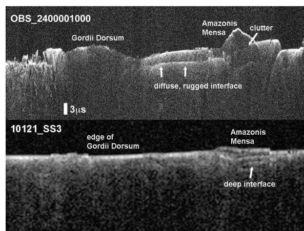
Fig. 3: SHARAD (top) and MARSIS data of Amazonis Mensa, from overlapping tracks (shown in Fig. 1). The MARSIS data has been adjusted to have north on the left to better compare to the SHARAD track. Note that the two tracks intersect in Amazonis Mensa, but do not cross the same terrain (Fig. 1). Therefore, they do not exactly match. A deeper interface is visible in the MARSIS data beneath Amazonis Mensa.
