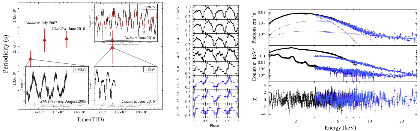
Figure 3. Left: period determination for the longest available archival X-ray observations, with the superimposed light curve binned at 1 ks bin -1 . Middle: energy-dependent, folded light curve for the simultaneous Chandra (black) and NuSTAR (blue) observations soon after the 2016 burst. Right: simultaneous spectral fit of the Chandra (black) and NuSTAR (light and dark blue) data with two absorbed blackbodies and a power-law component. The background spectrum is also plotted in the middle panel.
