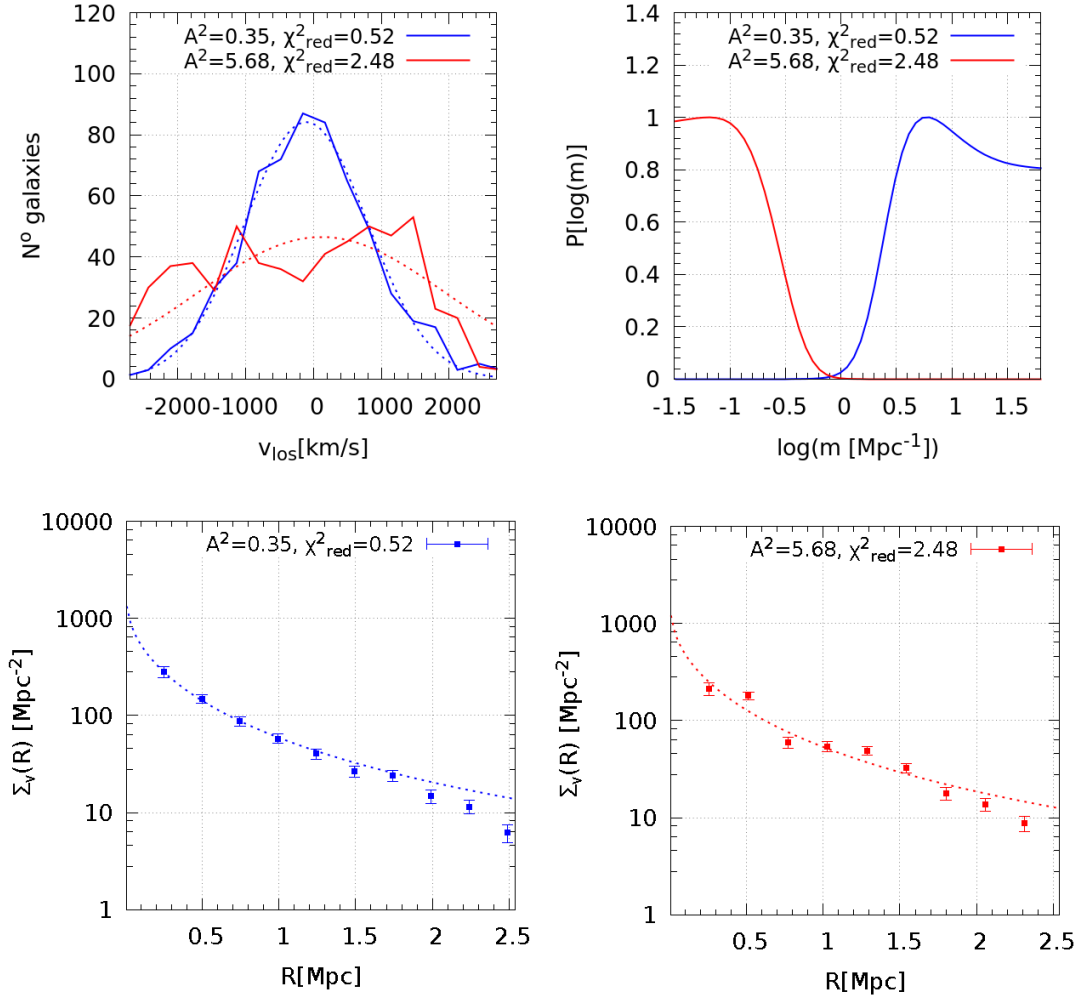
Figure 7. Upper left plot: line of sight velocity distributions of two projected phase spaces characterized by a large and a small value of A^2 , \chi^2_{red} (red and blue solid curves respectively). The dashed lines shows the best fit gaussians in the two cases. Upper right plot: corresponding distributions P[\log(m)] obtained by applying MG-MAMPOSSt procedure on these projected phase spaces assuming a "T" velocity anisotropy model in the fit. Lower plots: projected binned number density profiles (points with errorbars) and best fit pNFW profiles (dashed lines) obtained with the method of ref. [54]. Left: small values of A^2 , \chi^2_{red} . Right: large values of A^2 , \chi^2_{red} .
