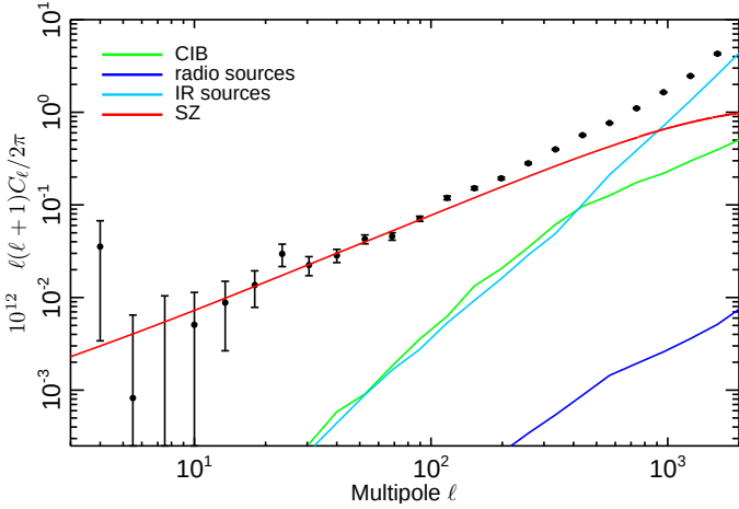
Fig. 34. Thermal SZ power spectrum from Planck data. Black points with errors show the C_\ell spectrum formed from the all-sky y map of Planck Collaboration XXII (2016) . Blue, green, and cyan lines represent a set of physically motivated foregrounds, with red being the best-fit SZ model from that paper.
