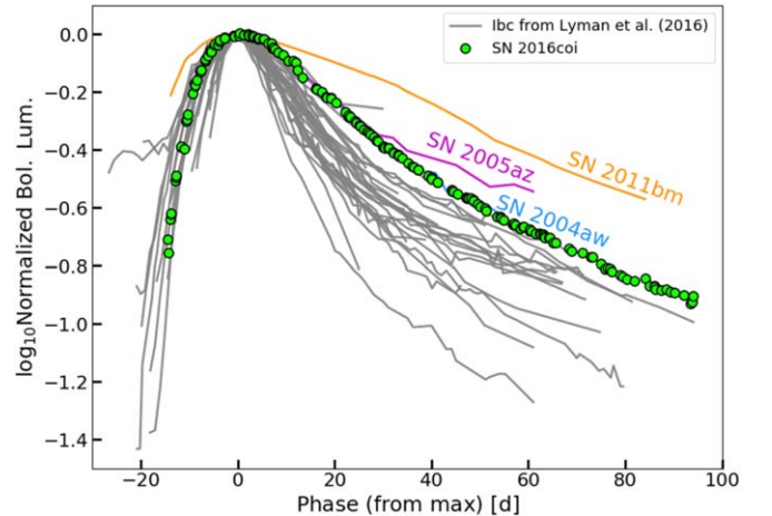
Figure 3. Comparison of the uvoir bolometric light curve of SN 2016coi with the sample of SESNe from Lyman et al. (2016). The light curves have been normalized to maximum light. SN 2016coi is among the objects with the broadest light curve, suggesting a larger-than-average diffusion time. The broad light curves of SNe 2004aw (which lies exactly below SN 2016coi; Taubenberger et al. 2006), 2005az (Drout et al. 2011), and 2011bm (Valenti et al. 2012) are also marked.
