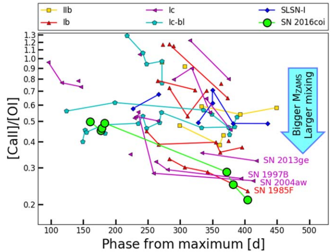
Figure 11. Comparison between the evolution of the [Ca II] \lambda\lambda 7291, 7324 to [O I] \lambda\lambda 6300, 6364 ratio for SN 2016coi and other Type Ib and Ic SNe. SN 2016coi is characterised by low [Ca II]/[O I] ratio, suggesting a high M_{\text{ZAMS}} progenitor, with a high level of mixing at the time of explosion. Other events with a low ratio are SNe 1985F, 1997B, and 2004aw. Measurements were performed depending on availability of late-time spectra retrievable from the literature (Filippenko & Sargent 1986; Gaskell et al. 1986; Filippenko et al. 1995; Barbon et al. 1999; Patat et al. 2001; Foley et al. 2003; Elmhamdi et al. 2004; Taubenberger et al. 2006, 2009; Tanaka et al. 2009; Milisavljevic et al. 2010, 2015a, 2015b; Benetti et al. 2011; Valenti et al. 2011, 2012; Silverman et al. 2012; Ben-Ami et al. 2014; Modjaz et al. 2014; Ergon et al. 2015; Kuncarayakti et al. 2015; Smartt et al. 2015; Drout et al. 2016; Nicholl et al. 2016; Kangas et al. 2017; Taddia et al. 2019).
