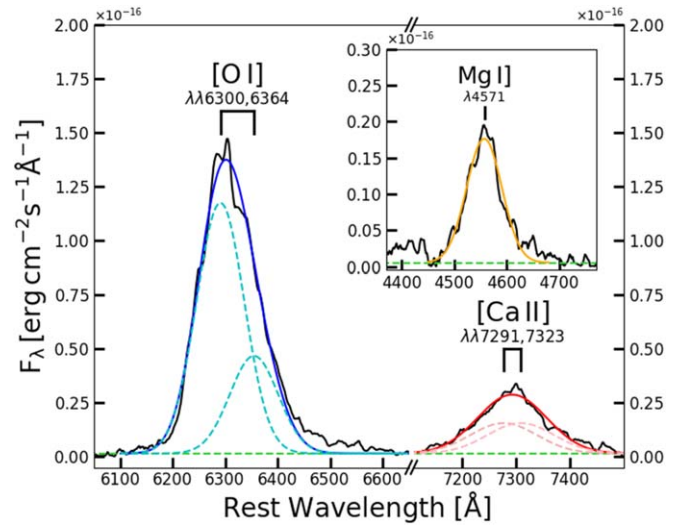
Figure 5. A zoomed-in plot of the spectral region of the [O I] \lambda\lambda 6300, 6364 , [Ca II] \lambda\lambda 7291, 7323 and Mg I \lambda 4571 lines of the MMT+BlueChannel nebular spectrum acquired on 2017 June 28 ( \sim 400 days after explosion). Gaussian profiles have been used to reconstruct the doublet components of the emission features. The observed lack of asymmetry of the [O I] emission feature might result from spherically symmetric ejecta, or possibly from an axisymmetric explosion, viewed at an angle below 50^\circ .
