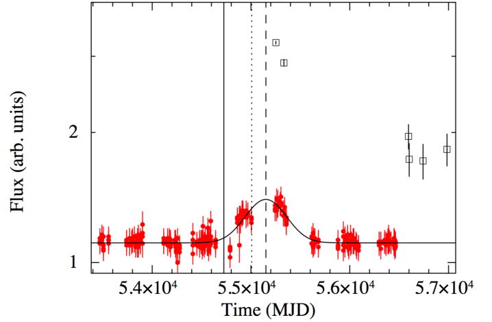
Fig. 4. Optical (flux) light curve of IC 3599 from the Catalina sky survey in arbitrary units (red dots), together with the Swift /XRT light curve (open squares) converted into flux using the spectral fit model, in arbitrary units. The Gaussian fit refers to the optical data. The vertical dashed line marks the time (MJD) of the optical peak, the dotted line the peak of the X-ray flux according to the multi-peak modelling. The continuous line marks the time at which the optical light curve rises by 10% from the quiescent level.
