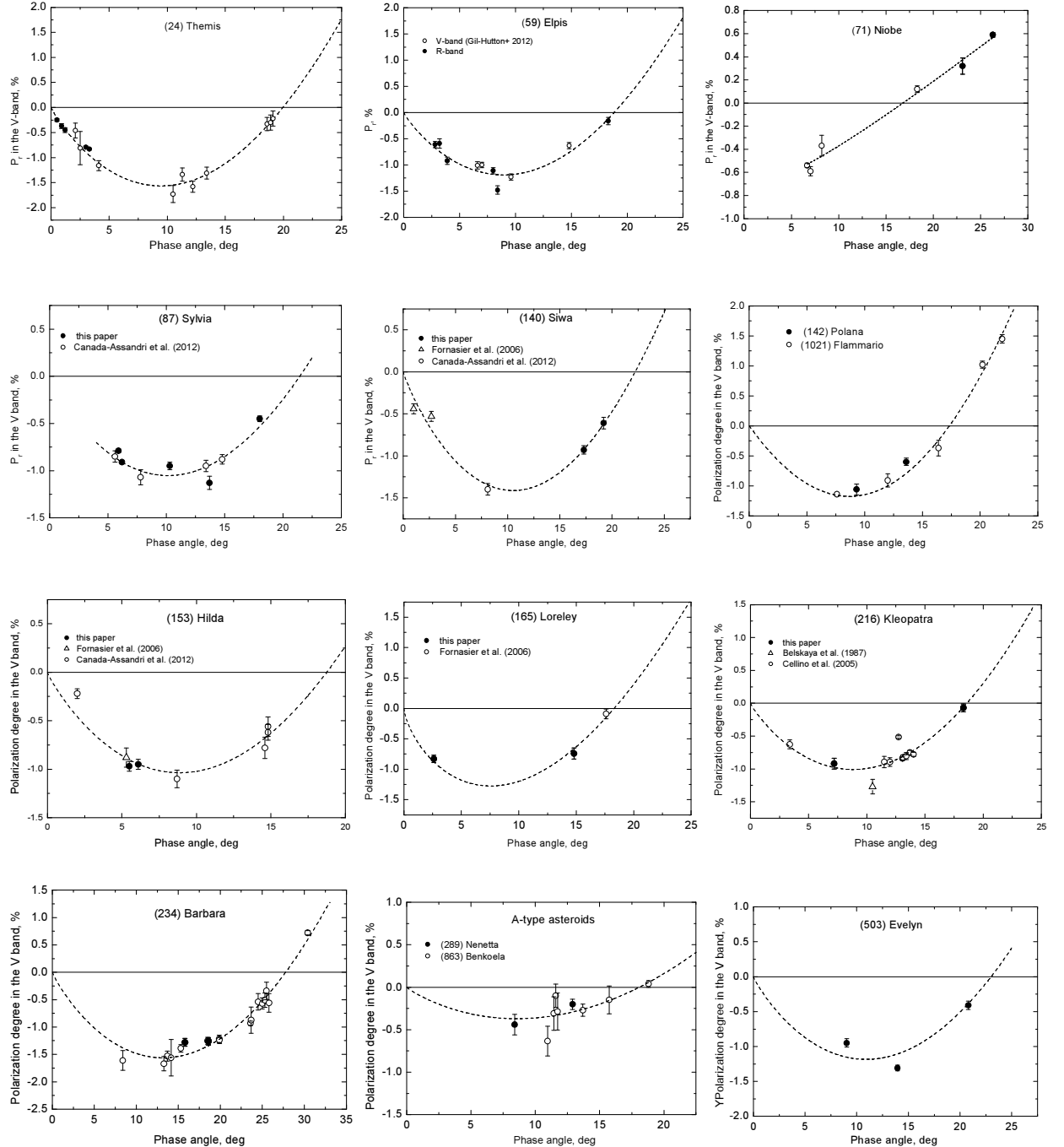
Fig. 1. The polarization-phase curve of the measured asteroids. New observations are shown by filled symbols and previously published data are shown by open symbols. Note that in some cases we mix together data taken in V and in R light. The corresponding references for each asteroid are given in the text. The dash lines shows the fit to the Lumme and Muinonen function.
