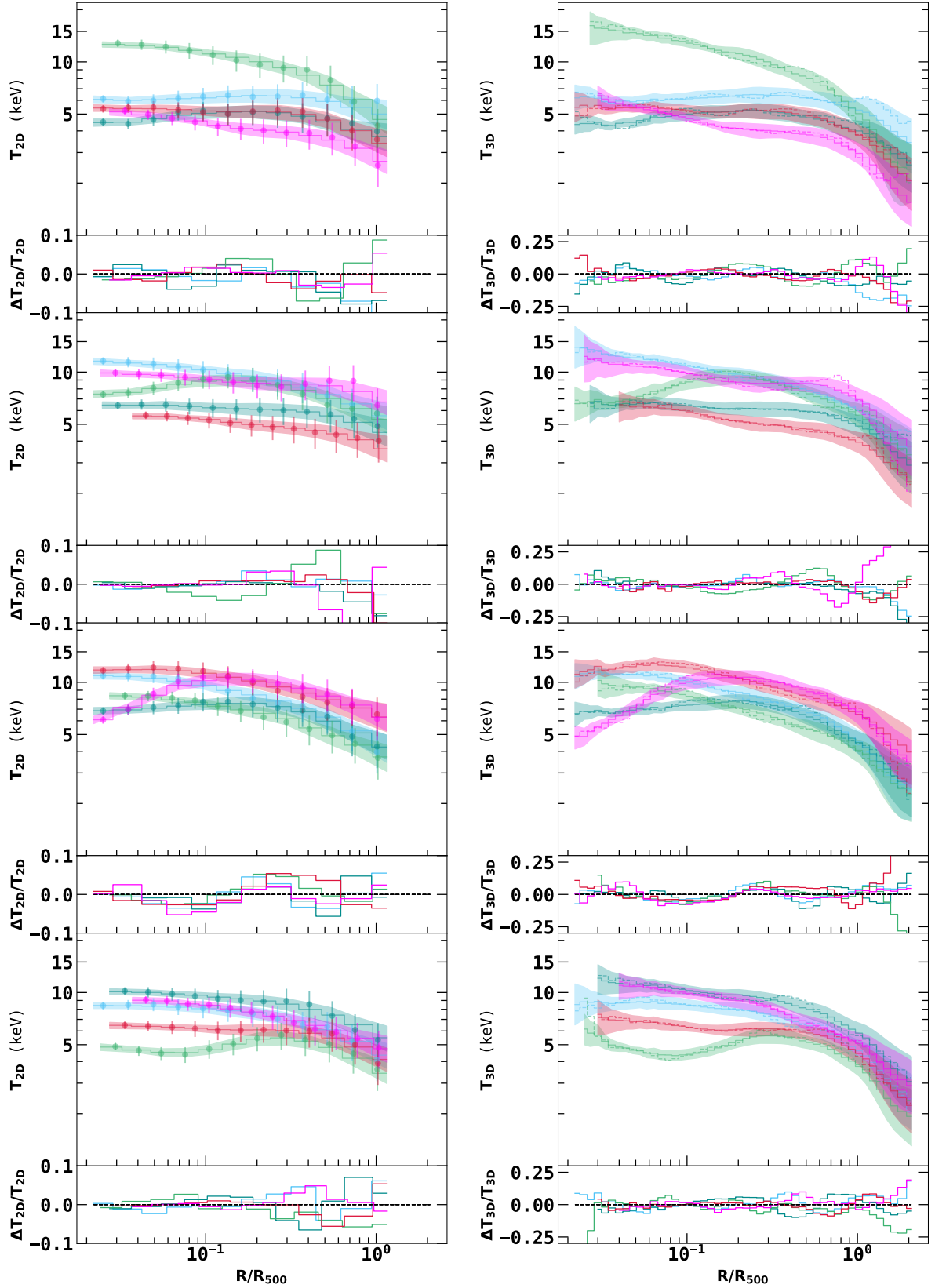
Fig. A.7. Left panel: Comparison of the 20 simulated 2D temperature profiles (solid points with errors) and reconstructed 2D temperature profiles obtained using IAE model (solid lines), the fitting being performed in the range [0.02-1] R_{500} considering twelve 2D temperature bins. The shaded regions represent the 1-\sigma dispersion of the reconstructed 2D temperature profiles. The smaller subplots show the residuals of the fit. Right panel: Solid lines and the shaded regions show the corresponding reconstructed 3D temperature profiles and the 1-\sigma dispersion respectively. Also shown in the dashed lines are the true 3D mass-weighted temperature profiles.
