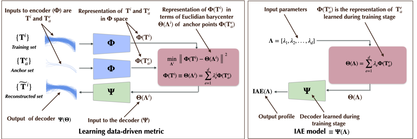
Fig. 6. Design of the neural network used in this work. Left Panel: Neural network used in the training stage. \Phi and \Psi represent the encoder and decoder respectively. T^i are the elements of the training set and T_a^e are the elements of the anchor set. \Phi(T^i) and \Phi(T_a^e) are the representations of T^i and T_a^e , respectively, in the encoder (feature) space. \Theta(\Lambda^i) = \Theta([\lambda_1^i, \dots, \lambda_d^i]) is the Euclidean barycentric representation of \Phi(T^i) in terms of d anchor points \Phi(T_a^e) , which is fed to the decoder. \Psi(\Theta) is the reconstructed output of the decoder. The network is trained by minimising the error between the input T^i and output \Psi(\Theta) temperature profiles. Right panel: Neural network (IAE model) of temperature profiles, where \lambda_1, \dots, \lambda_d are the input parameters and \text{IAE}([\lambda_1, \dots, \lambda_d]) is the output temperature profile. The decoder is not required in any step here.
