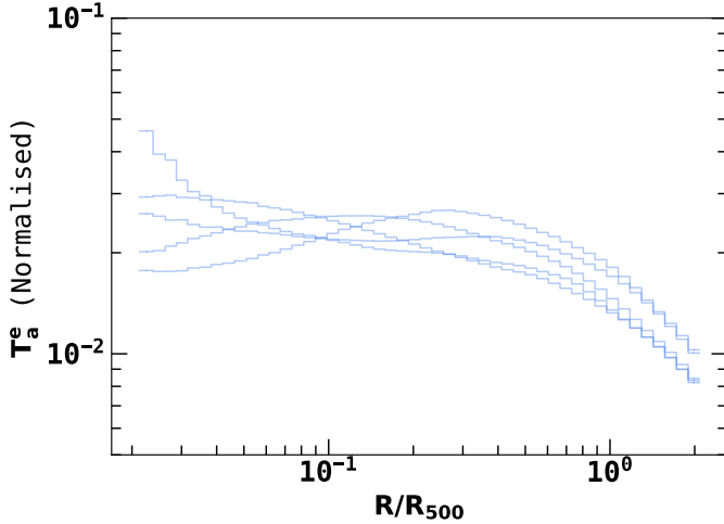
Fig. 7. Five anchor points (example profiles), T_a^e , where e runs from 1 to 5 used in the IAE model.
