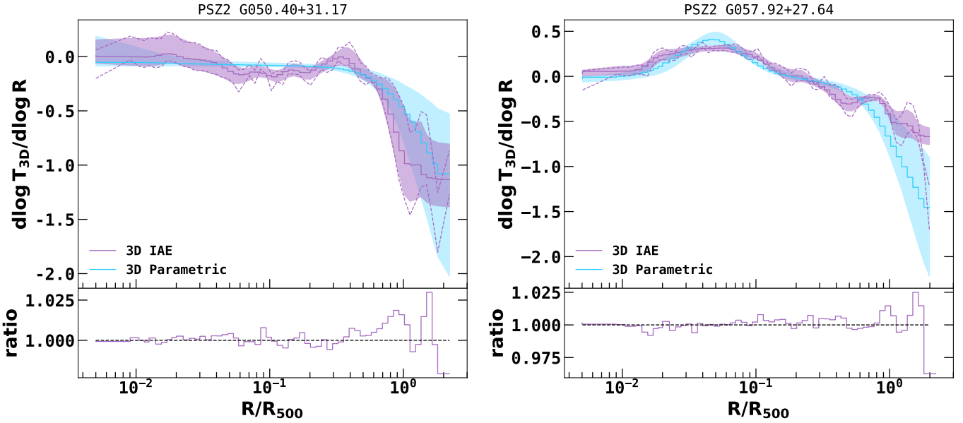
Fig. 21. Comparison of the logarithmic derivatives 3D temperature profiles of a typical NCC (PS22 G050.40+31.17) and CC (PS22 G057.92+27.64) cluster in the DR1 sample recovered with the IAE and parametric models. Solid lines and the associated shaded regions show the median and 1-\sigma dispersion obtained with MCMC. The region enclosed by the dashed lines represents 1-\sigma dispersion, if no smoothing is applied to the profiles derived from the MCMC chain. The bottom panel shows the ratio of the median 3D temperature profiles obtained using IAE with and without smoothing.
