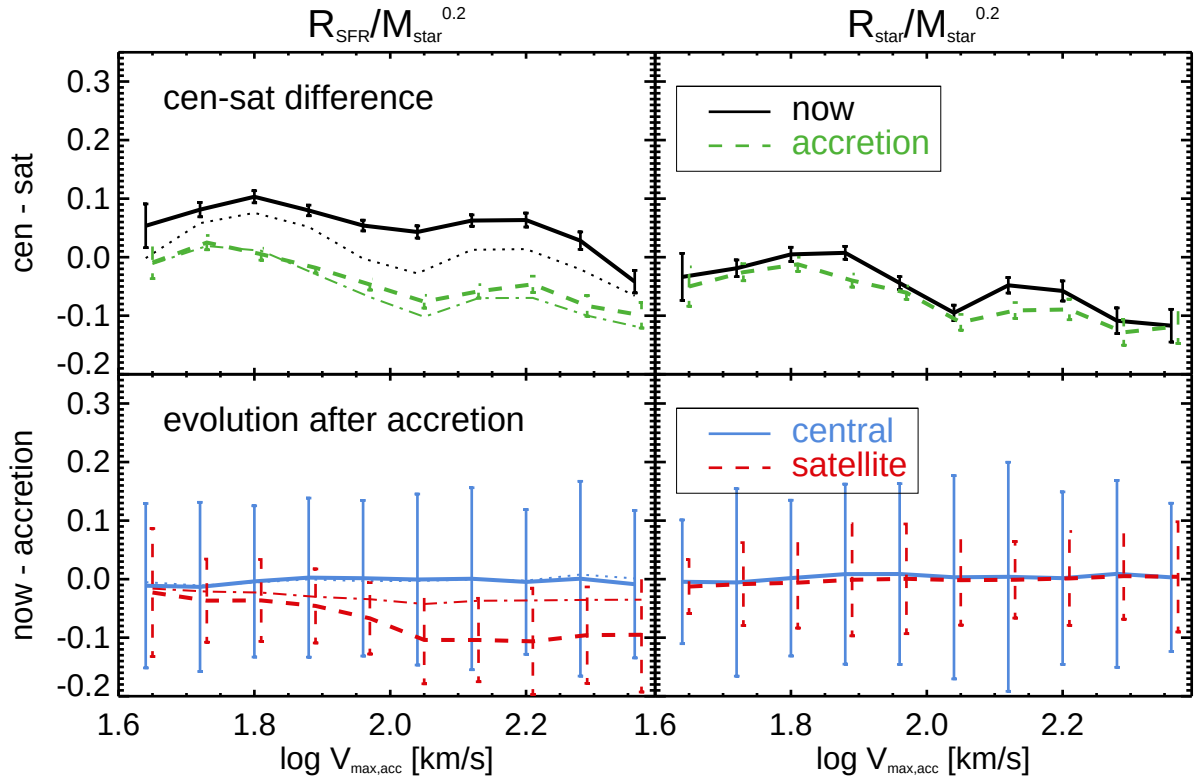
Figure 8. Top panels show the differences between the normalized SF (left) and stellar (right) radii of central and satellite galaxies at present (black solid) and at accretion time (green dashed). In the left panel, black dotted and green dot-dashed lines show the differences for the gaseous disc radii. Bottom panels show the differences between the properties predicted at present and at the time of accretion. Solid blue and dashed red lines correspond to central and satellite galaxies, respectively. Blue dotted and red dot-dashed lines show results for gaseous disc radii of central and satellite galaxies.
