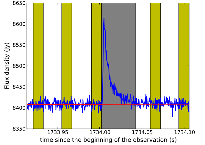
Figure 1. Dedispersed time series for the strongest giant pulse in the MWA data. The yellow (lighter) portions were used to estimate the off-pulse baseline shown by the red line. The gray (darker) area is the region that was integrated over to measure the total pulse energy. The plot spans 180 ms and has a time resolution of 400 \mu\text{s} .
