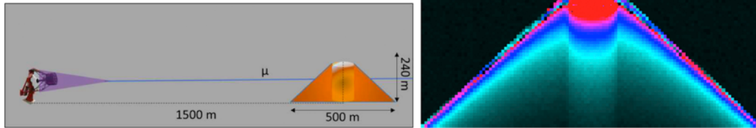
Fig. 3. Left: sketch of the telescope-volcano configuration used for our simulations. Despite Cherenkov light is produced along the whole muon path, we show only the one useful for our ASTRI-like telescope, i.e. that produced in the last 100 m. Right: a hollow conduit of 100 m diameter is resolved in about 9 nights by the muon radiography performed with the ASTRI-like telescope.
