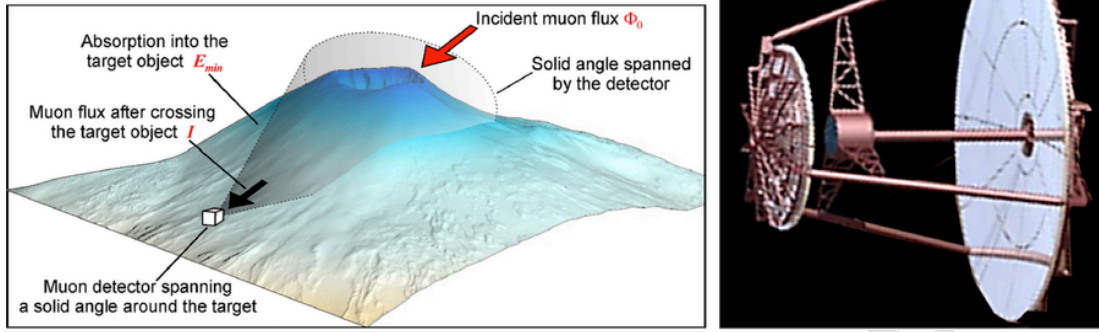
Fig. 1. Left: sketch of the muon radiography principles (from [6]). Right: schematic representation of a IACT with its main components. The primary mirror (right), optical camera (middle), secondary mirror (left) are shown.
