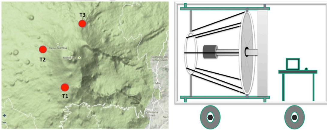
Fig. 4. Left: a possible configuration of the three different positions of the telescope around the SE crater to perform the Mt. Etna tomography. Right: sketch of a possible instrumentation.
