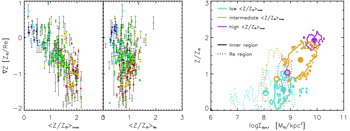
Figure 5. Left: Metallicity Z gradient against average stellar metallicity \langle Z/Z_{\odot} \rangle for galaxies in an inner region within 0.2 R_e (left) and in a R_e region within 0.8 - 1.0 R_e (middle). Colour coding is by galaxy morphological type, as in Figure 2. Right: Local metallicity Z against dynamically derived local surface mass density; contours cover spaxels with densities greater than 0.3 times the maximum density, for the inner region within 0.2 R_e , (solid lines and filled circles as mean points) and R_e region within 0.8 - 1.0 R_e , (dotted lines and open circles as mean points). Here different colors correspond to galaxies of different average central metallicity Z ; low ( \langle Z/Z_{\odot} \rangle_{\text{inner}} \sim 0 - 0.9 ; turquoise), intermediate ( \langle Z/Z_{\odot} \rangle_{\text{inner}} \sim 0.9 - 1.8 ; goldenrod) and high ( \langle Z/Z_{\odot} \rangle_{\text{inner}} \sim 1.8 - 4 ; purple).
