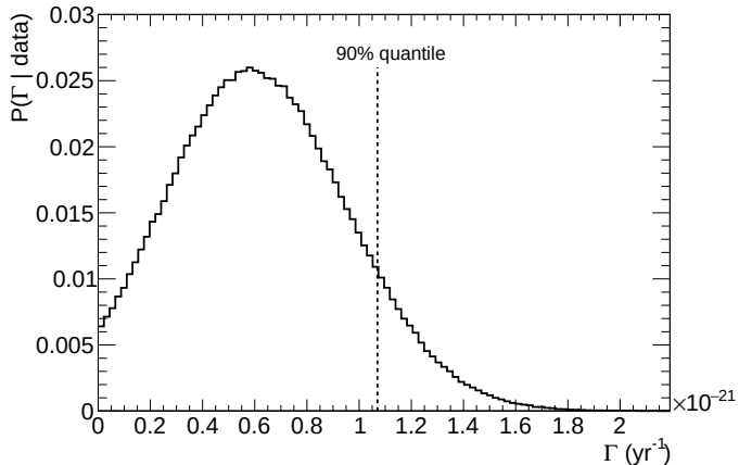
FIG. 3. Marginalized posterior probability distribution for the decay rate \Gamma . The vertical line indicates the 90% quantile from which the lower half-life limit was derived.
