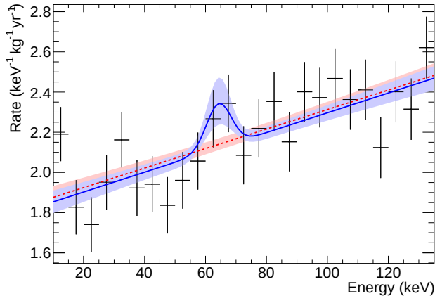
FIG. 2. Best fit to the data with the “signal+background” model f_{\text{sig}} (blue solid line) and the “background-only” model f_{\text{bkg}} (red dashed line). The shaded areas indicate the 68% uncertainty bands.
