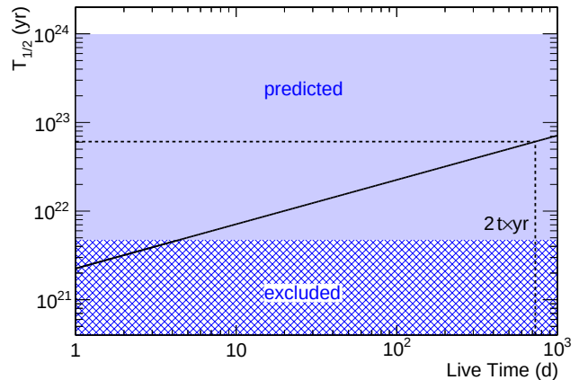
FIG. 4. Expected sensitivity of XENON1T for 2\nu 2K of ^{124}\text{Xe} assuming a 1 t fiducial volume. The blue-hatched area indicates the parameter space excluded by current experiments [23]. The blue shaded area shows the range of predicted half-lives [19].
