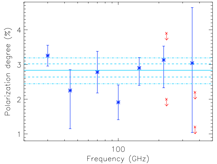
Fig. 2. Median polarization degrees for radio sources at Planck frequencies with their errors (blue data points), and upper limits (90% and 68% confidence) for dusty galaxies (red arrows). All values were corrected for the small biases discussed in Sect. 4.3. The solid blue line shows the minimum \chi^2 value of the median polarization degree of radio sources, assumed to be frequency independent. The dashed and dot-dashed lines show the 68% and 95% limits, respectively.
