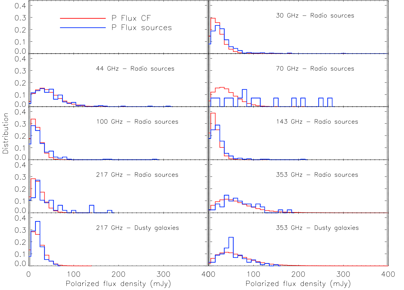
Fig. 1. Distribution of the polarized signals of PCCS2 radio sources and dusty galaxies compared with those of control fields (signals within a radius of FWHM/2 from the corresponding centers). The total flux density limits for radio sources are those listed in Table 7. For dusty galaxies at 353 GHz we have kept the same limit as for radio sources (784 mJy). At 217 GHz, S_{\text{lim,dusty}} = 300 mJy (see text).
